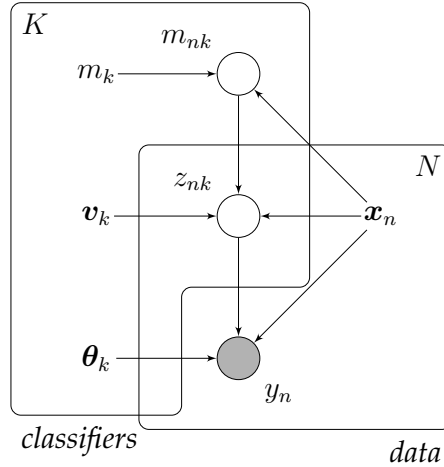
Figure 4.3: Directed graphical model of the generalised Mixture-of-Experts model. See the caption of Figure 4.1 for instructions on how to read this graph. When compared to the Mixture-of-Expert model in Figure 4.1, the latent variables z_{nk} depends additionally on the matching random variables m_{nk} , whose values are determined by the mixing functions m_k and the inputs \mathbf{x}_n .
