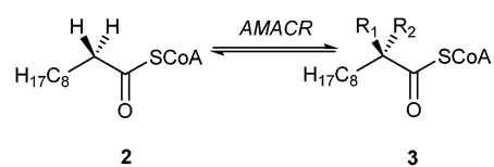
Scheme 2 Incorporation of deuterium during reaction of straight-chain fatty acyl-CoA esters (decanoyl-CoA 2 ) with AMACR ( R^1, R^2 = ^1\text{H} or 2 H).
