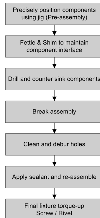
Figure 1: Generic Aerospace Assembly Process [9]
