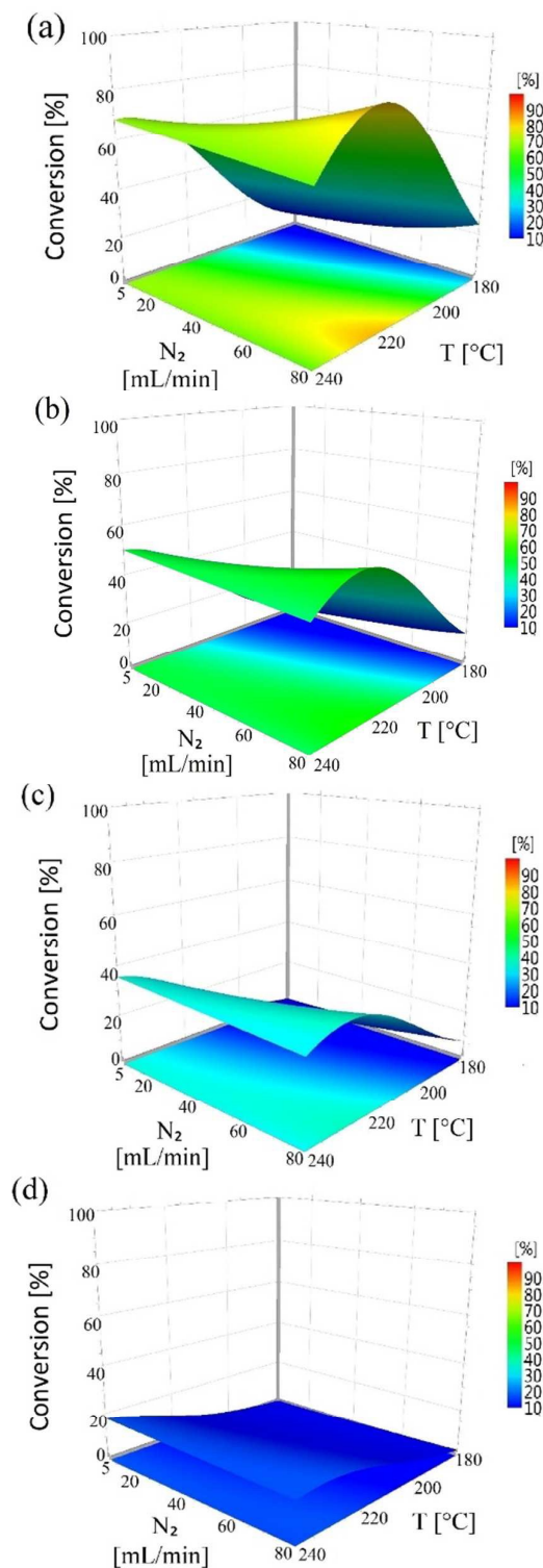
Fig. 3 Influence of temperature (180 – 240 °C) and nitrogen flow (5 – 80 mL/min, 33.3 - 566.7 \text{ m}^3 \text{ m}^{-2} \text{ h}^{-1} at STP) on conversion of substrate (10 wt%) for liquid feed flows of (a) 0.1 mL/min ( 0.7 \text{ m}^3 \text{ m}^{-2} \text{ h}^{-1} at STP), (b) 0.2 mL/min ( 1.4 \text{ m}^3 \text{ m}^{-2} \text{ h}^{-1} at STP), (c) 0.4 mL/min ( 2.7 \text{ m}^3 \text{ m}^{-2} \text{ h}^{-1} at STP), and (d) 0.5 mL/min ( 3.3 \text{ m}^3 \text{ m}^{-2} \text{ h}^{-1} at STP), in
