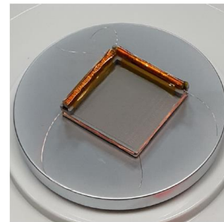
Figure 11. Three magnetorquers orthogonally mounted.
