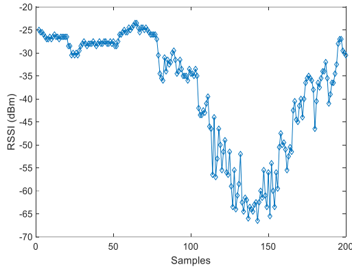
Figure 9. RSSI changes with distance between Femto-sat and a ground station.
