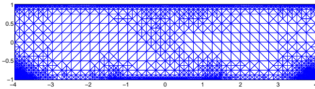
Figure 4.12.: Triangulation after 7 steps of the adaptive algorithm.
