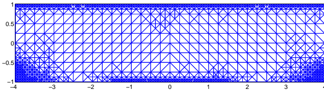
Figure 4.11.: Triangulation after 5 steps of the adaptive algorithm.
