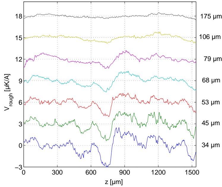
Figure 6.9: Roughness potential V_{\text{rough}}(z) for different heights of the cloud above the wire. Each curve is shifted successively about 3 \mu\text{K}/\text{A} to the top for better visibility.
