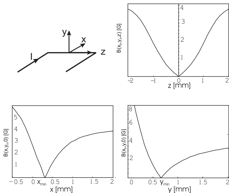
Figure 5.6: Magnetic fields created by the u-wire with a current of 2 A in the wire and an external magnetic field of 4.2 G in x-direction. The three graphs show the absolute value of the magnetic field in the three directions in space. Around the minimum, the field can be approximated by a linear function.
