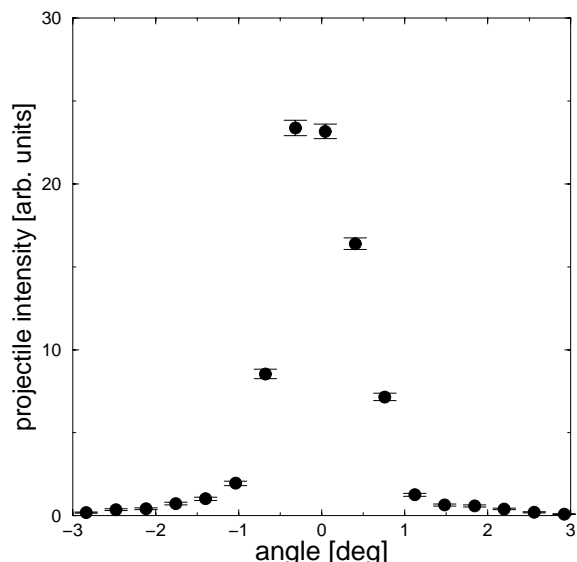
Figure 2.9: Profile of the projectile beam. Full width at half maximum is 1.3^\circ which includes the angular resolution of the detection aperture of 0.7^\circ .
