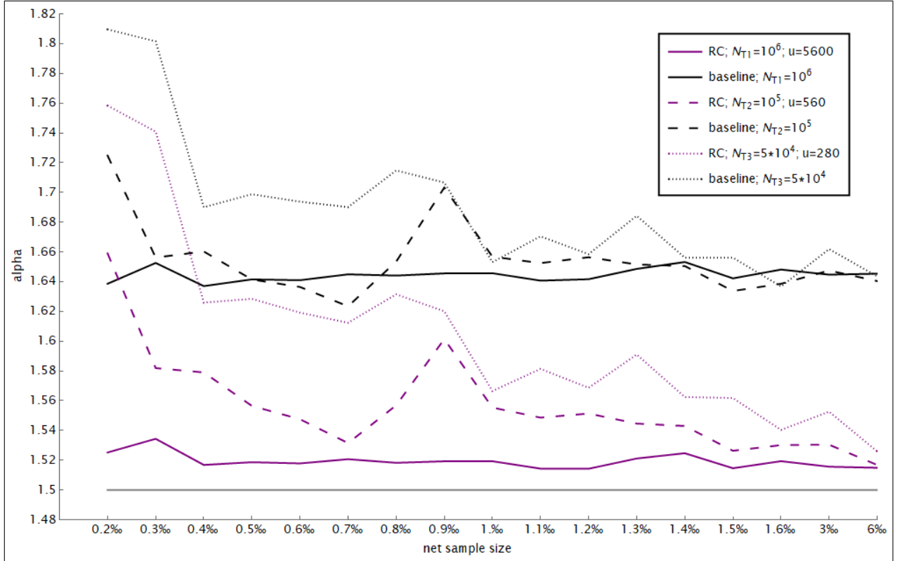
Population sizes of N_{T1} = 10^6 , N_{T2} = 10^5 and N_{T3} = 5 \cdot 10^4 are used together with accordingly scaled correction factors: u = 5600 , u = 560 and u = 280 .
