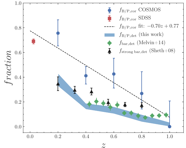
Figure 13. Fraction of barred galaxies with B/P bulges corrected for unfavourable inclinations and bar orientations in our sample, as well as changing resolution, S/N and bandshifting, using equation (4) (blue circles for COSMOS and red square for SDSS). The trend declines with increasing redshift, showing the genuine evolution in the B/P fraction. The dashed line shows a linear fit to the mean, binned, corrected B/P fractions, from z \approx 0 to z = 1 . For comparison, the detected B/P bulge fraction ( f_{B/P, \text{det}} ) is shown with the blue band. The detected fractions of disc galaxies with strong bars in COSMOS from Sheth et al. (2008) (black triangles) and Melvin et al. (2014) (green diamonds) are also represented. The error bars in f_{B/P, \text{cor}} show the combined uncertainties on f_{B/P, \text{det}}(z) ( 1\sigma limits in the binomial confidence interval, shown in Fig. 7) with the uncertainties in the coefficients of the logistic regression fitted to the REDSHIFTED-control sample (parameters shown in Table 1) and propagated using equation (4).
