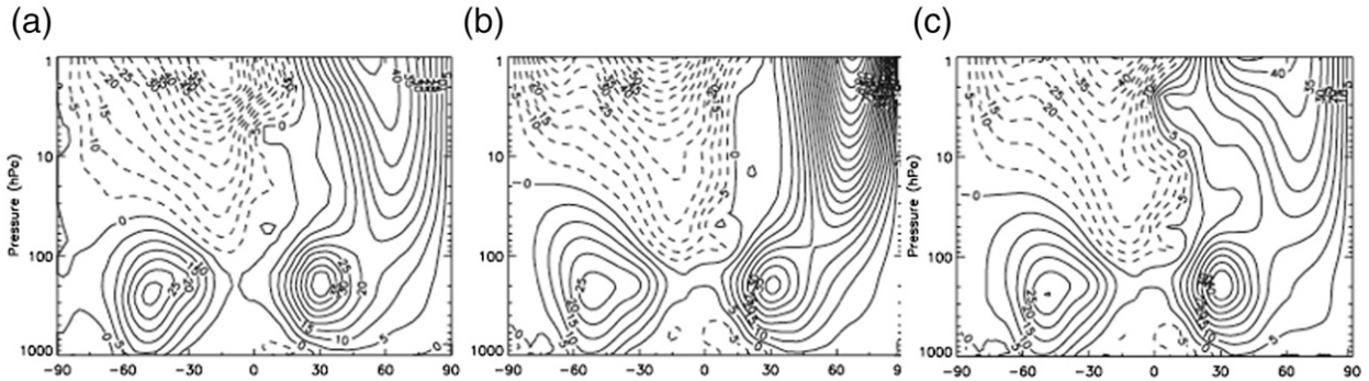
FIG. 27-3. (a) Climatological January zonally averaged zonal-mean wind as a function of pressure altitude and latitude (positive indicates north) for 1980–99 from the ERA-40 reanalysis dataset. (b) As in (a), but from a GISS model with no gravity wave parameterization. (c) As in (b), from the same GISS model with a gravity wave parameterization included. [Panels (a) and (b) are from Fig. 1 and (c) is from Fig. 6 of Geller et al. (2011).]
