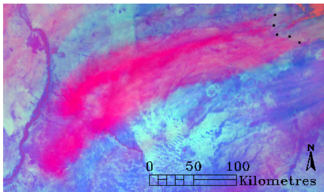
Figure 2. VIIRS Dust RGB (Lensky and Rosenfeld, 2008) showing dust being emitted northeast of the Sudanese Nile (latitude 18^\circ , longitude 35^\circ ) on 19 December 2016. Dust point source locations are identified by tracking dust plumes back to their first point of occurrence.
