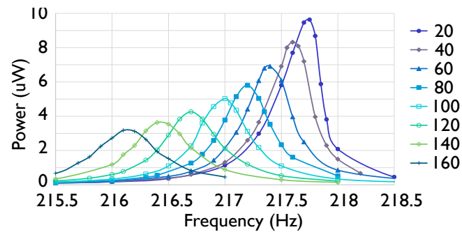
Figure 4. Experimental power as a function of input frequency, for several temperatures.
