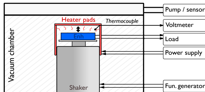
Figure 3. Schematic diagram of the experimental setup.
