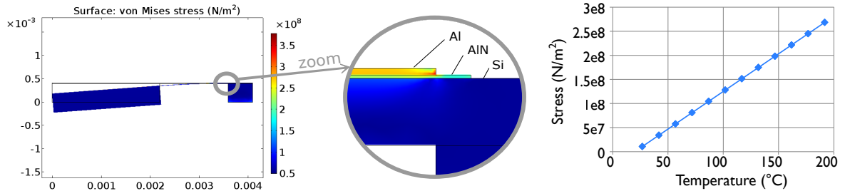
Figure 6. Comsol simulation of the thermal stresses when the cantilever is subjected to 150 °C, and average stress as a function of the temperature.
