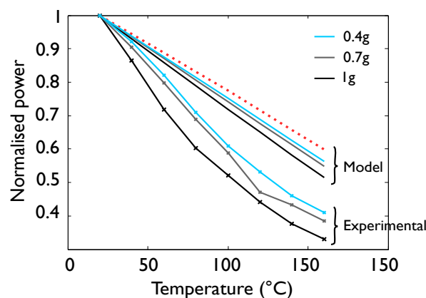
Figure 7. Normalized power as a function of temperature, modeled and experimental data for three different input acceleration.
