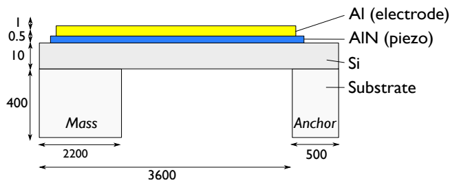
Figure 1. Schematics of the cantilever, dimensions in \mu\text{m} .
