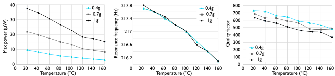
Figure 5. Experimental maximum power, resonance frequency and quality factor as a function of input temperature.
