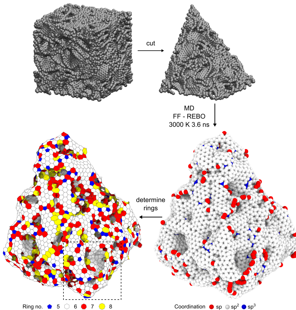
Figure 2: Protocol for preparing the molecular geometry. A three dimensional periodic model prepared using the REBO forcefield [8] was used from de Tomas et al. [12]. The corner was cut and the surface was annealed using the same forcefield for 3.6 ns at 3000 K to anneal the surface. The structure is shown coloured by the coordination number (2 - red, 3 - white, 4 - blue). The different rings were then determined and are coloured according to ring number (5 - blue, 6 - white, 7 - red, 8 - yellow). Dashed box around the region is shown expanded in Figure 7
