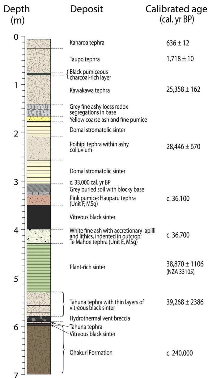
Fig. 8. Stratigraphy of deposits in the hill adjacent to the Meade trench. Ages of the tephras and the basal ignimbrite (Ohakuri Formation) are given in Table 2; the calibrated ^{14}\text{C} -age for plant-rich sinter is from this study. The base of the domal stromatolitic sinter at ~3 m depth is estimated to be aged c. 33,000 cal. yr BP, assuming that the underlying paleosol represents ~3000 years of development on Hauparu tephra (based on Lowe and Hogg, 1995). MSg, Mangaone Subgroup (Jurado-Chichay and Walker, 2000, 2001; Nairn, 2002).
