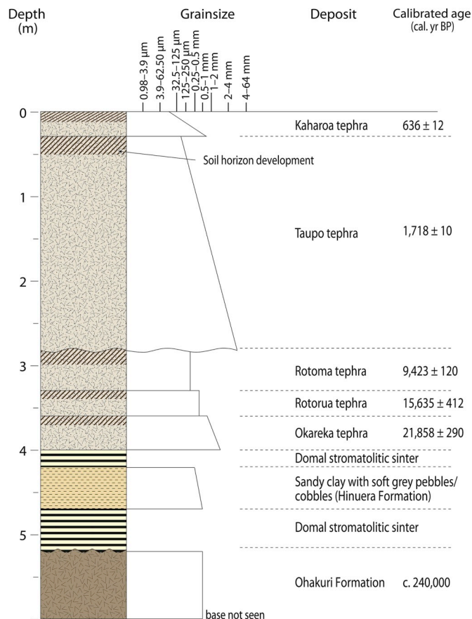
Fig. 5. General stratigraphy of the Meade trench and ages of tephra and other deposits. Paleosols occur in the upper parts of each tephra; modern soil horizons are formed on Kaharoa tephra. Grain sizes depicted are from field observations. Ages are from sources listed in Table 2. The sediments of the Hinuera Formation are assumed to be aged between c. 25.4 cal. ka (i.e., younger than Kawakawa tephra/Oruanui Formation) and c. 21.8 cal. ka (Okareka tephra).
