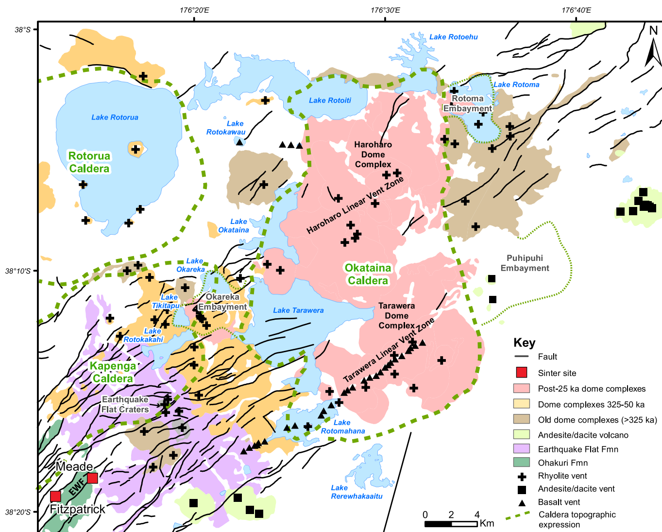
Fig. 13. Simplified volcanic geology of the Okataina Volcanic Centre including lava dome complexes (all of which were deposited in association with multiple pyroclastic eruptives: Nairn, 2002) and their general ages, and locations of the main faults. The northern part of the adjacent Kapenga Volcanic Centre, which hosts the Ngakuru Graben and the Meade study site just to the southwest (Fig. 1E), is also indicated. EWF, East Whirinaki Fault. After Nairn (2002), Leonard et al. (2010), and Cole et al. (2014).
