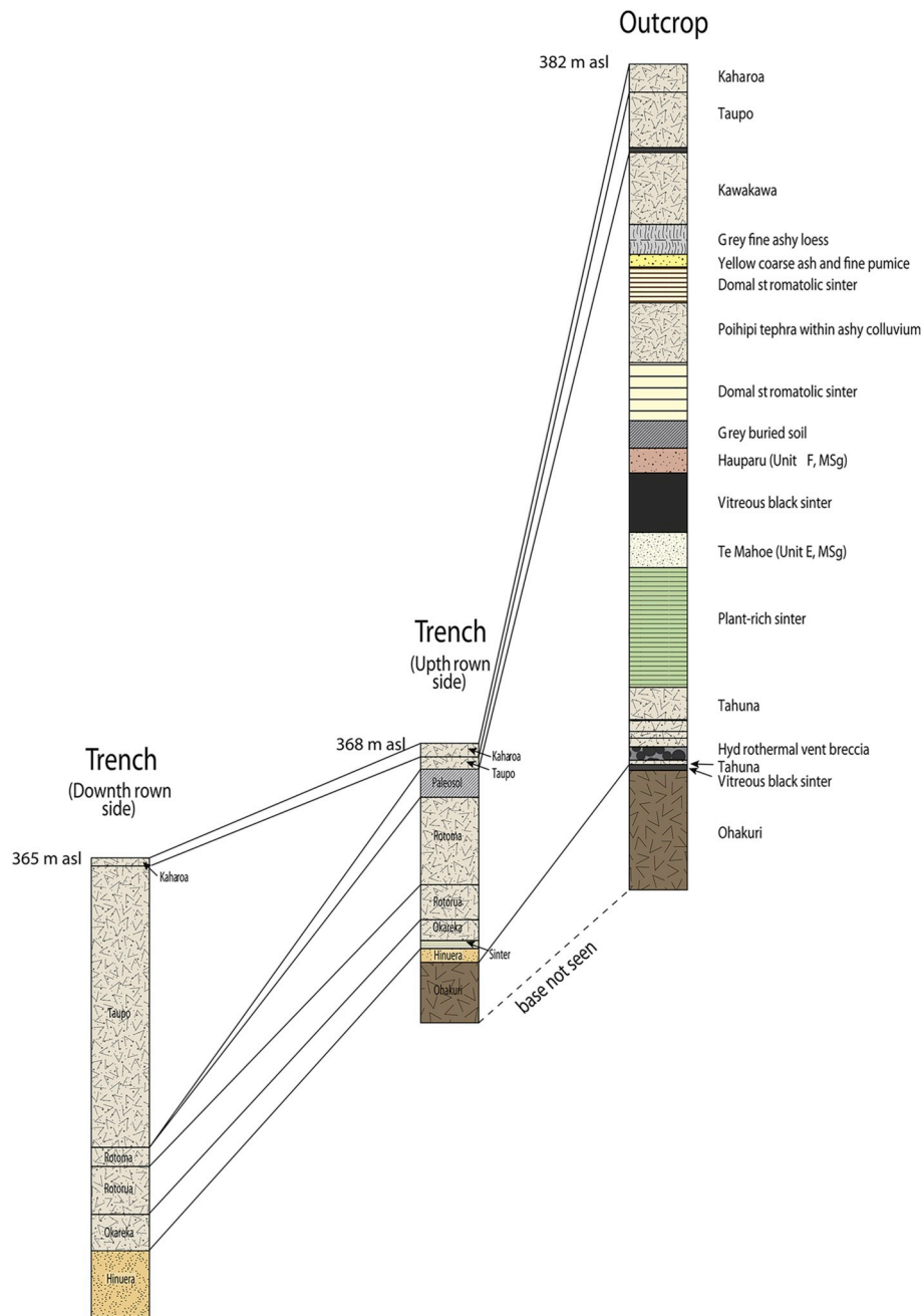
Fig. 9. Correlation of units (Kaharua and Taupo tephras, a domal stromatolitic sinter, and Ohakuri Formation) in the Meade trench and in the outcrop on the shoulder-slope of the adjacent hill.
