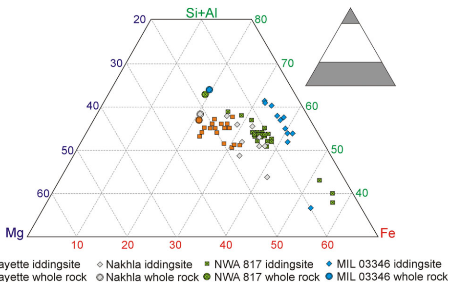
Fig. 8. Bulk chemical compositions of four of the nakhlites and their iddingsite (atom%). The bulk rock data were sourced as follows: Lafayette (Boctor et al. 1976), Nakhla (mean of analyses in McCarthy et al. 1974; Dreibus et al. 1982; Anand et al. 2005), NWA 817 (Sautter et al. 2002), and MIL 03346 (mean of analyses in Anand et al. 2005; Day et al. 2006). The iddingsite analyses plotted have been obtained by SEM-EDX or electron probe and so will average the compositions of different intergrown generations (e.g., NWA 817 low- and mid-Z iddingsite). The iddingsite data were sourced as follows: Lafayette (Bunch and Reid 1975; Boctor et al. 1976; Treiman et al. 1993; Bridges and Grady 2000; Vicenzi et al. 2002; Kuebler et al. 2004; Changela and Bridges 2011; Tomkinson et al. 2013; Hicks et al. 2014), Nakhla (Bunch and Reid 1975; Gooding et al. 1991; Changela and Bridges 2011; Hallis et al. 2012, 2014; Hicks et al. 2014; Lee et al. 2013, 2015a; Lee and Chatzitheodoridis 2016; Goodrich et al. 2013), NWA 817 (Gillet et al. 2002; Sautter et al. 2002; Hicks et al. 2014; the present study), and MIL 03346 (Day et al. 2006; Sautter et al. 2006; Imae and Ikeda 2007; Hallis and Taylor 2011; Kuebler 2013; Hallis et al. 2014; Hicks et al. 2014). (Color figure can be viewed at wileyonlinelibrary.com .)
