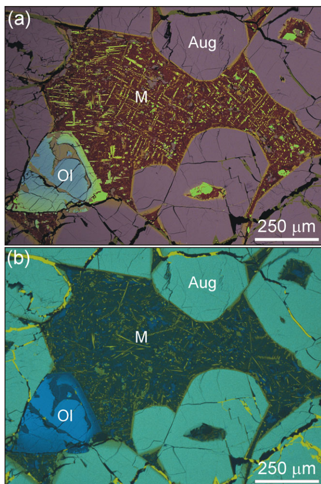
Fig. 1. An area of N8-1 containing augite (Aug), olivine (Ol), and mesostasis (M). a) X-ray map overlain on a BSE image. The X-ray map has been made by blending three element maps: Si K\alpha (red), Mg K\alpha (blue), and Fe K\alpha (green). These color combinations render augite grain cores purple, the narrow Fs-rich rims to augite grains orange, olivine grain cores blue, olivine grain rims light green, iddingsite brown, equant grains of Fe-Ti oxide lime green, and the mesostasis predominantly dark red. Both the augite and olivine grains are compositionally zoned, and the mesostasis contains many acicular Fe-rich crystals. b) X-ray map of the same field of view as (a) that was made by blending maps for Mg K\alpha (blue) and Ca K\alpha (yellow). This element combination renders olivine mid blue to dark blue, augite turquoise, calcite yellow. Open fractures are black, and the mesostasis contains a variety of fine crystals. Note that the calcite veins are almost entirely restricted to augite. (Color figure can be viewed at wileyonlinelibrary.com .)
