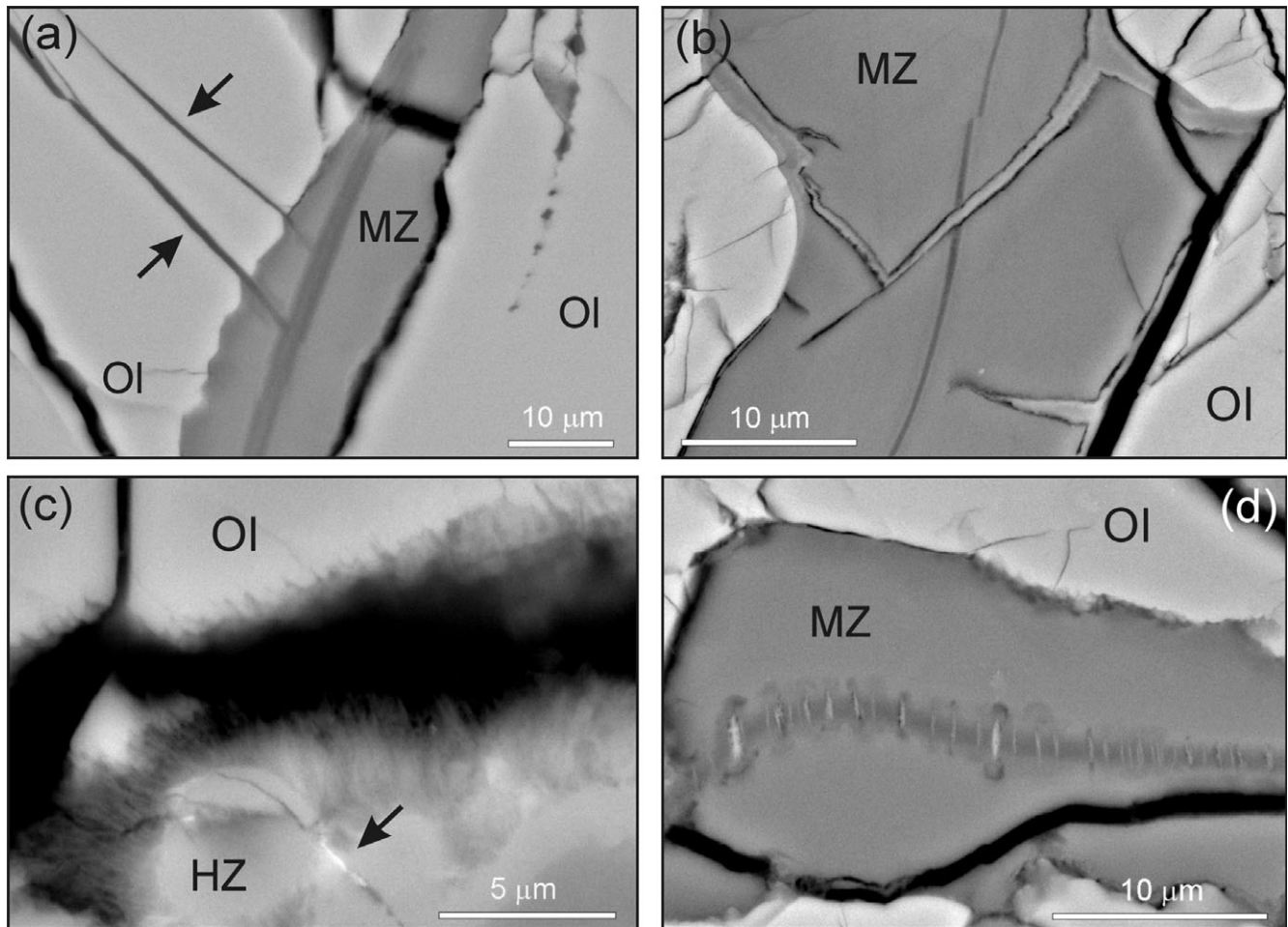
Fig. 5. BSE images of iddingsite veins within olivine (Ol) phenocrysts from N8-1. a) The vein in the center of the image has an axial band of low-Z iddingsite that is flanked by mid-Z iddingsite (MZ). A pair of narrow low-Z veins (arrowed) extend from the left-hand side of the axial band into olivine. b) A vein containing a low-Z axial band, mid-Z iddingsite (MZ), and high-Z iddingsite. The high-Z component occurs as a selvage between mid-Z iddingsite and olivine, and as veins that crosscut mid-Z iddingsite and the axial band. c) The interface between high-Z iddingsite (HZ) and the olivine vein wall, along which is a fracture (black). Fine fibers project from high-Z iddingsite across the fracture and into olivine. Barite (white) occurs within the high-Z iddingsite (arrowed). d) A vein that is dominated by mid-Z iddingsite (MZ) whose axial band (dark gray) is crosscut by needles of high-Z iddingsite that together make a ladder-like texture.
