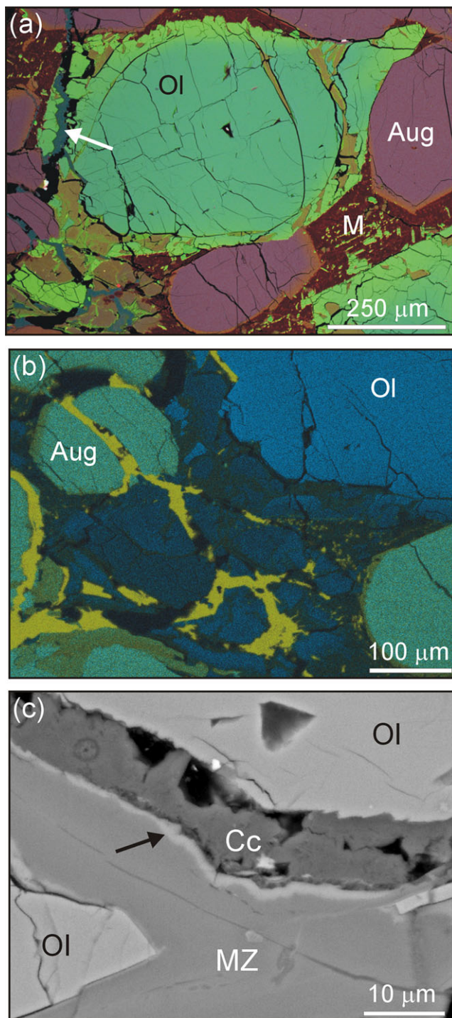
Fig. 4. An altered phenocryst of olivine (Ol) in N8-1. a) X-ray map overlain on a BSE image. The X-ray map has been made by blending three element maps: Si K\alpha (red), Mg K\alpha (blue), and Fe K\alpha (green). These color combinations render augite (Aug) grain cores purple, the narrow Fs-rich rims to augite grains dark orange, olivine grain cores light blue, olivine grain rims light green, iddingsite brown, calcite dark blue-green (indicated by white arrow), and the mesostasis (M) predominantly dark red. Iddingsite veins occur mainly in outer parts of the olivine grain core and in its rim. b) X-ray map of an area in the lower left hand corner of (a) that was made by blending maps of Mg K\alpha (blue) and Ca K\alpha (yellow). This element combination renders olivine mid blue to dark blue, augite turquoise, and the anastomosing veins of calcite yellow. c) BSE image of a vein of calcite (Cc) that occurs between mid-Z iddingsite (MZ) and olivine. High-Z iddingsite (light gray selvage indicated by a black arrow) occurs between mid-Z iddingsite and calcite, whereas the contact between olivine and mid-Z iddingsite in the lower left hand side of the image has very little high-Z iddingsite. (Color figure can be viewed at wileyonlinelibrary.com .)
