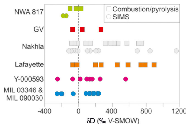
Fig. 9. Hydrogen isotopic composition of iddingsite in the nakhrites. The secondary ion mass spectrometry (SIMS) data are from Gillet et al. (2002) (NWA 817) and Hallis et al. (2012) (Y-000593, Nakhla, and the paired meteorites MIL 03346 and MIL 090030). The stepwise combustion/pyrolysis data are from the present study (NWA 817, Table 2) and Leshin et al. (1996) (Lafayette, Nakhla, Gobernador Valadares [GV]). \delta\text{D} values of all of the temperature steps are plotted. (Color figure can be viewed at wileyonlinelibrary.com .)
