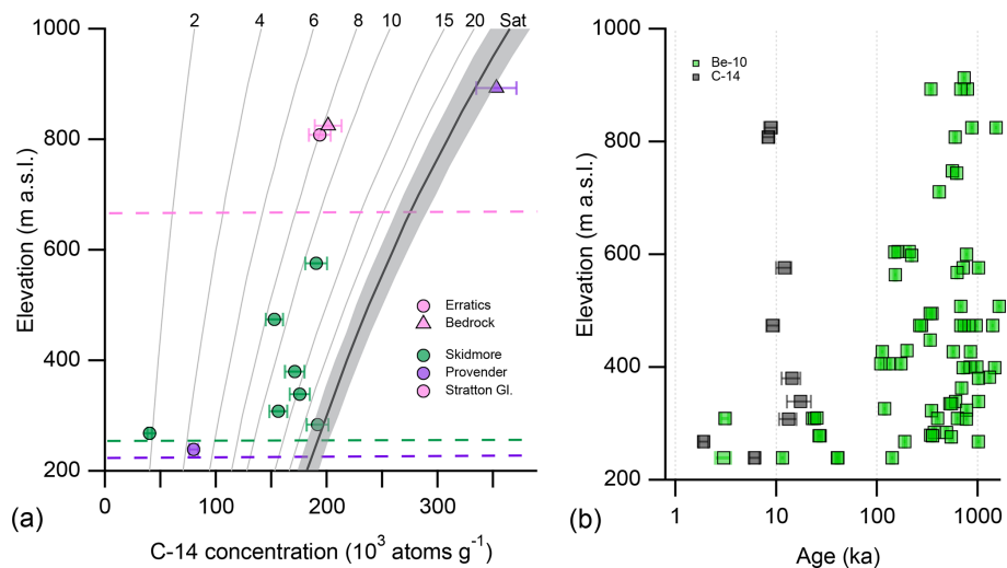
Figure 5. (a) Elevation versus in situ ^{14}\text{C} concentration of samples from the Shackleton Range. Circles are erratic cobbles; triangles are bedrock. Some error bars are smaller than their respective data points. Horizontal dashed lines show the approximate elevation of the modern ice surface at each site. Light grey lines indicate isochrons of exposure duration. Thick black line and grey shading are the saturation concentration and associated error envelope. (b) Exposure ages from this study (in situ ^{14}\text{C} ) and ^{10}\text{Be} ages of Hein et al. (2011, 2014). Samples yielding infinite in situ ^{14}\text{C} ages are not presented on the right-hand plot.
