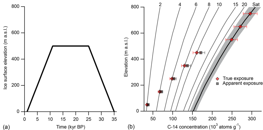
Figure 3. (a) Hypothetical ice surface elevation change at a nunatak partially covered by ice at the LGM. (b) Resulting in situ ^{14}\text{C} concentration, assuming no surface erosion, in samples collected at 100 m intervals along an elevation transect on the surface of the nunatak. Thin black lines indicate isochrons of exposure duration. Thick black line with grey shading represents the saturation concentration and associated error envelope. Error envelope represents typical analytical uncertainty. “True exposure” refers to the resulting ^{14}\text{C} concentration associated with the ice surface change history on the left plot. “Apparent exposure” is the resulting concentration that includes an inherited component, which is a residual ^{14}\text{C} inventory remaining from the hypothetical samples which were saturated prior to ice cover.
