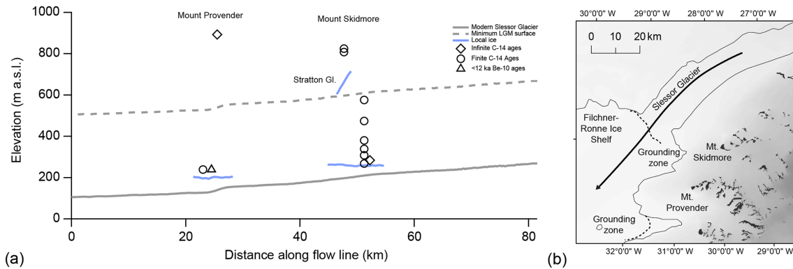
Figure 10. (a) Exposure-age results projected onto an elevation profile along flow line of the Slessor Glacier. (b) Flow line location is shown in the map. Infinite ^{14}\text{C} measurements are offset in regard to their distance along flow line to improve readability. The ^{10}\text{Be} data included are those from Hein et al. (2011, 2014) which yield exposure ages below 12 ka (LSDn scaling, http://antarctica.ice-d.org , last access: 2 November 2019). Elevation data for ice surfaces and map shading are sourced from the Reference Elevation Model of Antarctica (REMA; Howat et al., 2018). Grounding line positions sourced from the MEaSUREs program V2 (Rignot et al., 2011, 2014, 2016). Minimum LGM surface is the modern-day surface profile with the elevation increased above present using our minimum LGM thickness estimates.
