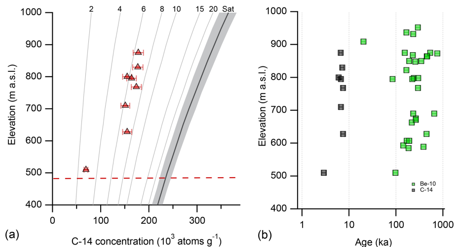
Figure 6. (a) Elevation versus in situ ^{14}\text{C} concentration of samples collected from the Lassiter Coast. All samples are bedrock. (b) In situ ^{14}\text{C} exposure ages with ^{10}\text{Be} ages of Johnson et al. (2019).
