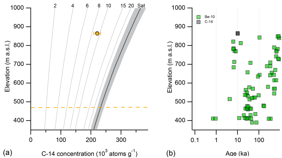
Figure 8. (a) Elevation versus in situ ^{14}C concentration of samples collected from the Thomas Hills. All samples are erratics. Note that both plots contain in situ ^{14}C data for two samples within close agreement, such that the points overlap. (b) Thomas Hills exposure ages from this study (in situ ^{14}C ) and those of Balco et al. (2016) and Bentley et al. (2017) ( ^{10}Be ).
