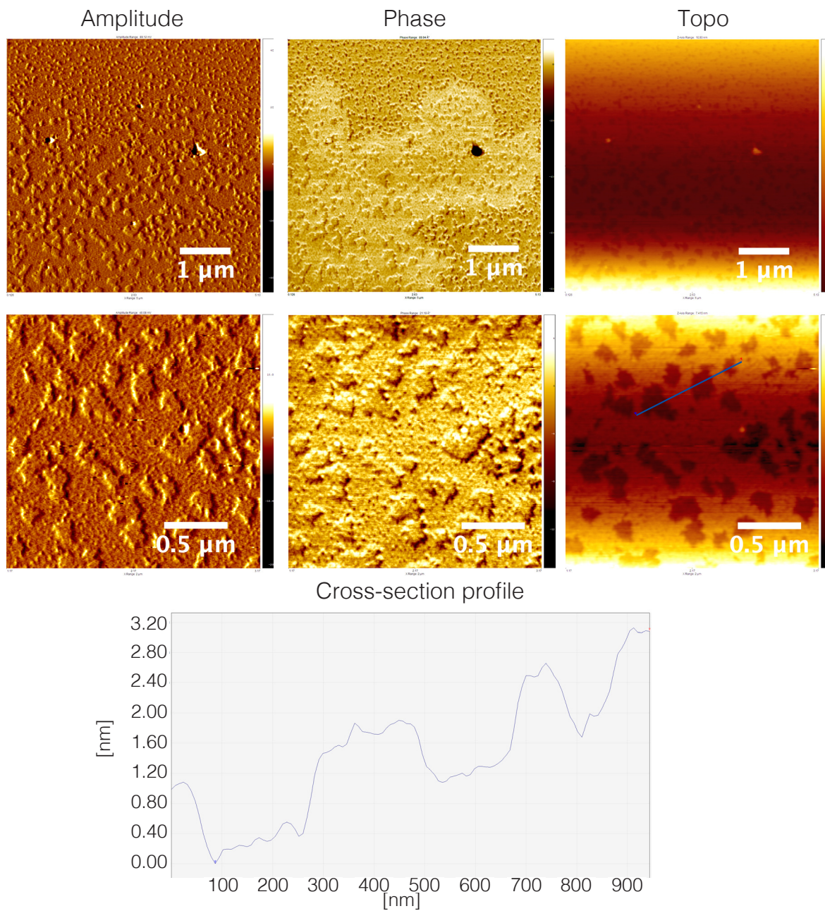
Figure S10. Amplitude-, phase-, and Z-axis-range AFM micrographs of \text{NH}_2\text{COOH-Y} and height-profile for cross-section indicated with blue line. Samples prepared from 2.5 \times 10^{-2} mg/mL in 10 \times 10^{-2} mM \text{NaCl} dilutions deposited on mica.
