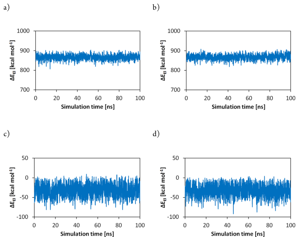
Figure S19. Electrostatic contribution for self-assembling a function of simulation time for NO 2 COOMe-Y (a), NH 2 COOMe-Y (b), NO 2 COOH-Y (c) and NH 2 COOH-Y (d).
