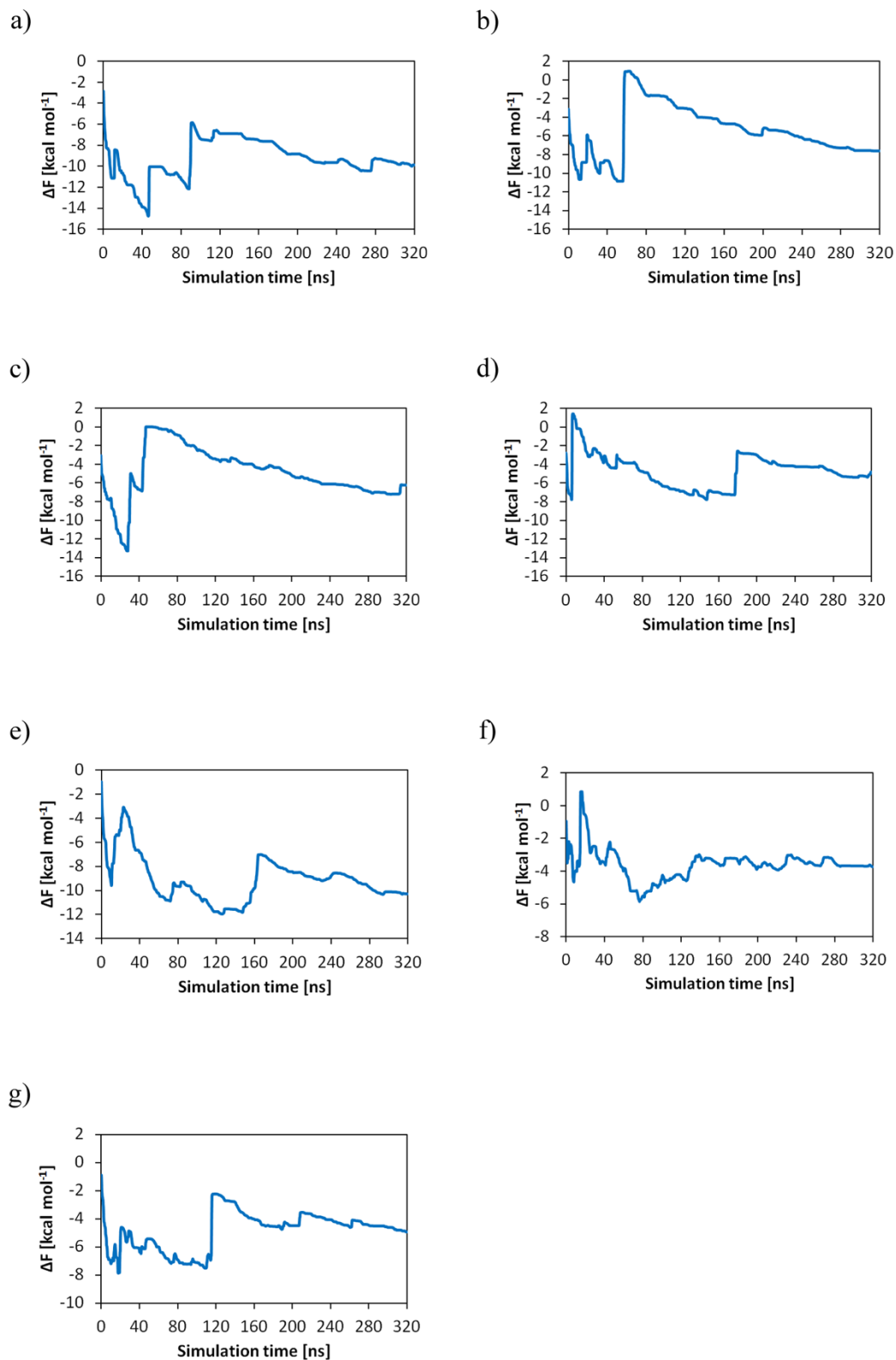
Figure S17. Free energy difference between bound and unbound state as a function of simulation time for \text{NO}_2\text{COOMe-Y} (a), \text{NH}_2\text{COOMe-Y} (b), \text{NO}_2\text{COOH-Y} (c), \text{NH}_2\text{COOH-Y} (d), \text{sym}(\text{COOMe})_2\text{-Y} (e), \text{short NO}_2\text{COOMe-Y} (f) and \text{NO}_2\text{ArCOOH-Y} (g).
