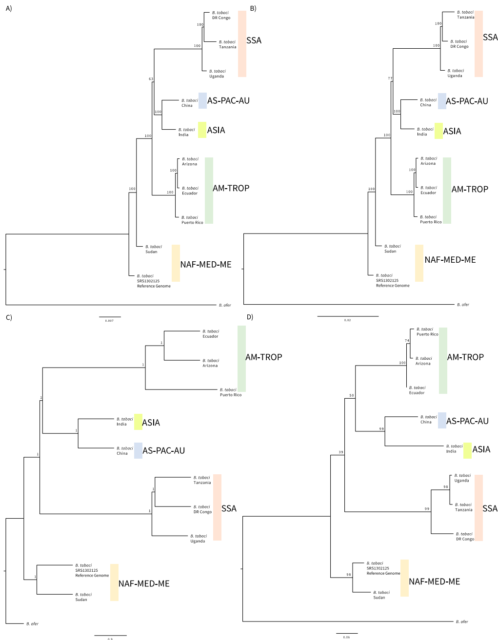
Figure 1. Colors correspond results suggested by automatic barcode gap discovery (ABGD) tests for putative species. (A) Result of the concatenated maximum likelihood (ML) analysis of all nucleotide sites from the nuclear supermatrix ( \ln\text{Likelihood} = -6919264.24 ). Scale bar represents substitutions per site. Clade values are depicted as bootstrap support. (B) Result of the partitioned ML analysis of the nuclear supermatrix ( \ln\text{Likelihood} = -6907791.99 ). Scale bar represents substitutions per site. Clade values are depicted as bootstrap support. (C) Result of ASTRAL coalescent analysis of 2184 gene trees. Scale bar represents coalescent units. Clade values are depicted as local posterior probabilities. (D) Result of ML analysis of cytochrome oxidase I (COI) sequences obtained from read-mapping ( \ln\text{Likelihood} = -6174.94 ). Scale bar represents substitutions per site. Clade values are depicted as bootstrap support.
