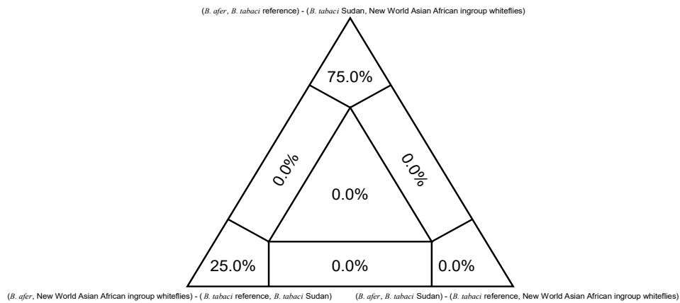
Figure 3. Likelihood map produced from IQ-tree showing the distribution of quartets that support a sister relationship between the reference “B” genome and the Sudan sample produced from the analysis of the concatenated alignment. Results show that 75% of quartets sampled support the Sudan sample together with the remaining samples (not including the reference) while 25% support the Sudan sample together with the reference, when all nucleotide sites are analyzed. These quartets are also relatively decisive in that no quartets provide ambiguous information (i.e., no points in the center or edges of the triangle).
