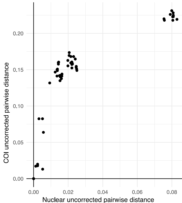
Figure 2. A scatter plot of uncorrected pairwise distances of COI versus uncorrected pairwise nuclear divergence for each whitefly specimen analyzed.
