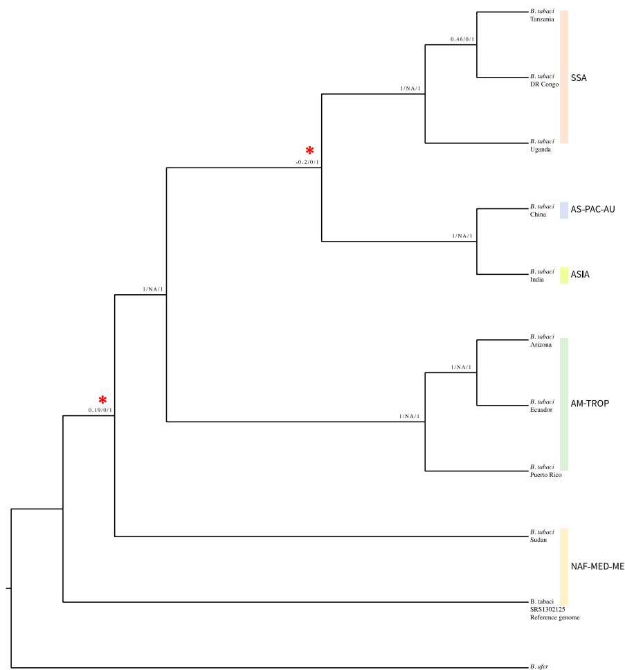
Figure 4. The B. tabaci complex of whiteflies showing the results of quartet sampling (QC: quartet concordance (frequency a concordant topology is observed)/QD: quartet differential (scaled fraction of discordant topologies)/QI: quartet informativeness (proportion of replicates that are informative)). Red asterisk indicate nodes of instability as discussed in the text. Nodes represented by 1/NA/1 are most stable and no discordant topologies are detected across quartets sampled (QD = NA).
