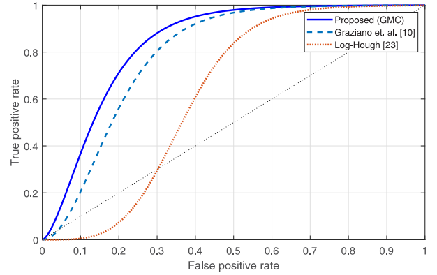
Fig. 6. Performance comparison in terms of ROC curves.
