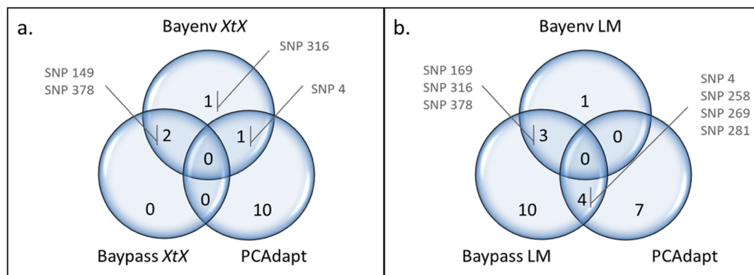
Figure 2. Venn diagrams comparing the outliers detected using PCAadapt with those identified using (a) the XtX statistics from Bayenv2 and Baypass, and (b) the Bayesian linear model (LM) from Bayenv2 and Baypass. Only the SNPs found under selection in more than one method are indicated.
