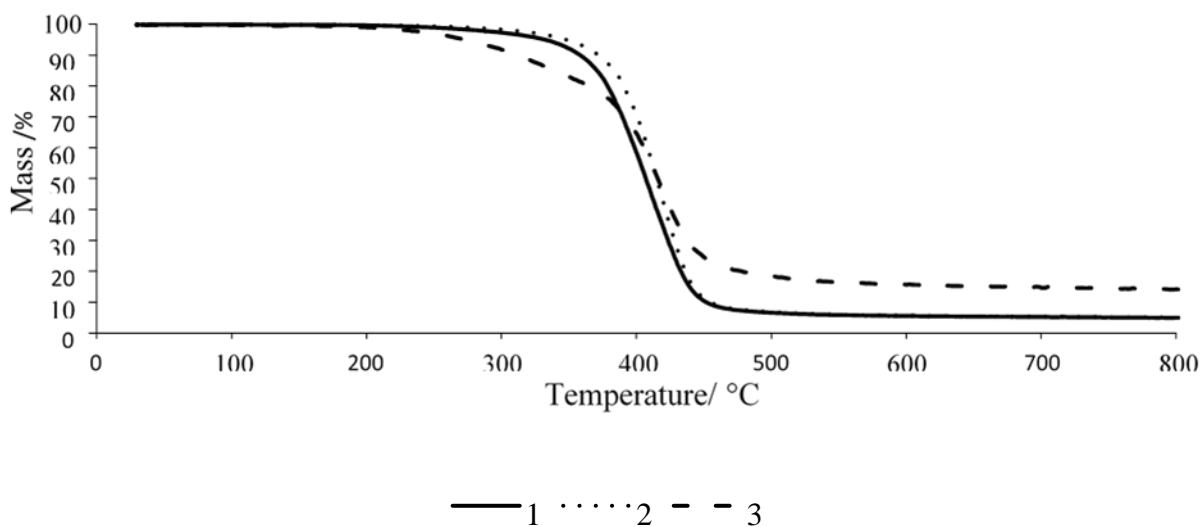
Figure 8. Thermogravimetric analysis (TGA) data for the three cured resin blends 1, 2, and 3.
