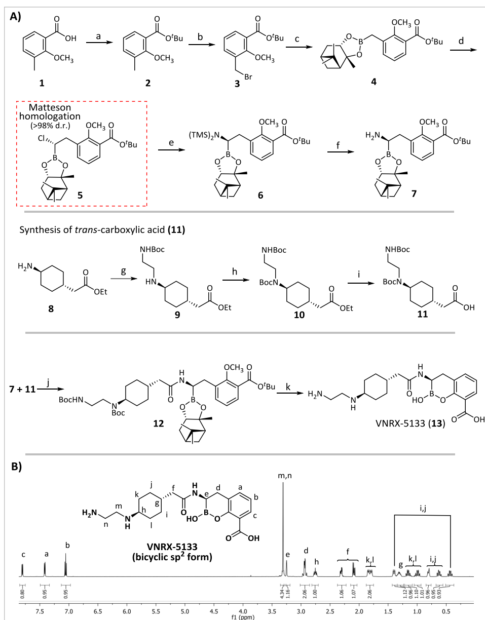
Figure 2. Synthesis and NMR analysis of VNRX-5133. (A) Reagents and conditions: (a) oxalyl chloride, cat. DMF, \text{CH}_2\text{Cl}_2 , room temperature (rt), 90 min and then 2-methylpropan-2-ol, 40^\circ\text{C} , 18 h; (b) N -bromosuccinimide, benzoyl peroxide, \text{CCl}_4 , reflux, UV, 5 h; (c) bis[ (+)-pinanediolato ]diboron, \text{Pd}(\text{dppf})\text{Cl}_2 , KOAc, 1,4-dioxane, 95^\circ\text{C} , 16 h; (d) \text{CH}_2\text{Cl}_2 , tetrahydrofuran (THF), n -BuLi, -100^\circ\text{C} , 45 min and then 4 in THF, \text{ZnCl}_2 , -95^\circ\text{C} to rt, overnight; (e) lithium bis(trimethylsilyl)amide, THF, -100^\circ\text{C} to -78^\circ\text{C} , 2 h; (f) MeOH, THF, -10^\circ\text{C} to rt, 1 h; (g) \text{K}_2\text{CO}_3 , 1:1 \text{CH}_2\text{Cl}_2/\text{H}_2\text{O} , rt, 1 h and then 2-( boc -amino)ethyl bromide, benzyltriethylammonium chloride, reflux, 18 h; (h) di- tert -butyl dicarbonate, N,N -diisopropylethylamine, reflux, 16 h; (i) \text{LiOH}\cdot\text{H}_2\text{O} , 1:2:1 THF/EtOH/ \text{H}_2\text{O} , rt, 5 h; (j) 11 , triethylamine, PyBOP and then crude 7 , rt, 75 min; (k) \text{BCl}_3 , \text{CH}_2\text{Cl}_2 , -78^\circ\text{C} , 1 h. (B) ^1\text{H} NMR (600 MHz) of high-performance liquid chromatography (HPLC)-purified VNRX-5133 in \text{D}_2\text{O} .
