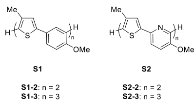
Figure 5. Monomers, dimers and trimers proposed for computational studies. The hexyl chains from the monomers 5 and 6 were replaced by methyl groups in S1 and S2 respectively, to reduce computational time. Further the end groups were replaced by a proton as the most neutral substituent.
