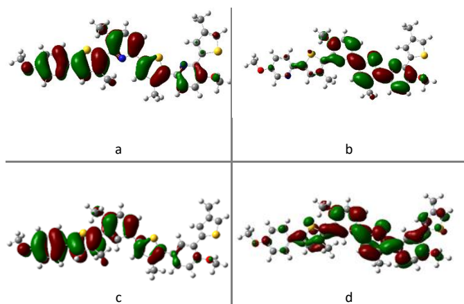
Figure 6. Molecular orbitals (displayed with an isovalue of 0.02), of trimer S1-3 : HOMO (a) and LUMO (b) and of trimer S2-3 : HOMO (c) and LUMO (d).
