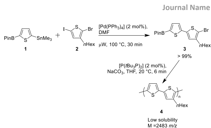
Scheme 2. Synthetic way to obtain a polymer based on a single monomer type M-Ar-Ar-X . 31
