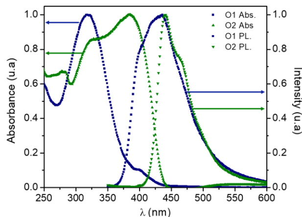
Figure 4. Normalized absorption spectra (abs.) and PL spectra of O1 and O2 ( \lambda_{\text{exc}} = 340 \text{ nm} ) in dichloromethane.
