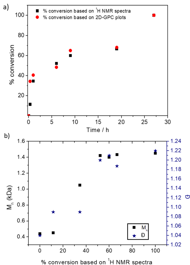
Figure 3. Plots of a) % conversion vs. time. Calculated by the two detectors ( ^1\text{H} and 2D-plots GPC) and b) M_n and \bar{D} vs. % conversion calculated by ^1\text{H} NMR; for the polymerization of 6 with 5 mol% of [\text{Pd}(\text{tBu}_3\text{P})_2] , 1.2 eq. CsF in THF at 50 °C. The conversion was calculated relative to compound 20 (product
