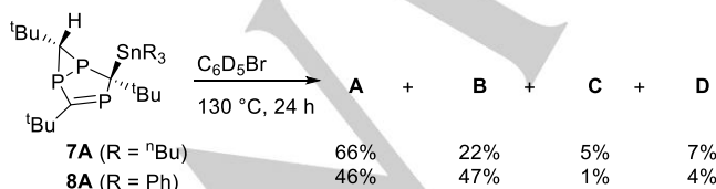
Scheme 5. Interconversion of 7A and 8A to diastereomers A-D at elevated temperatures
