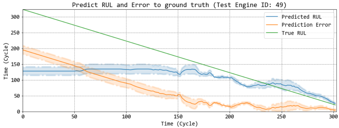
(a) 4-layer LSTM
