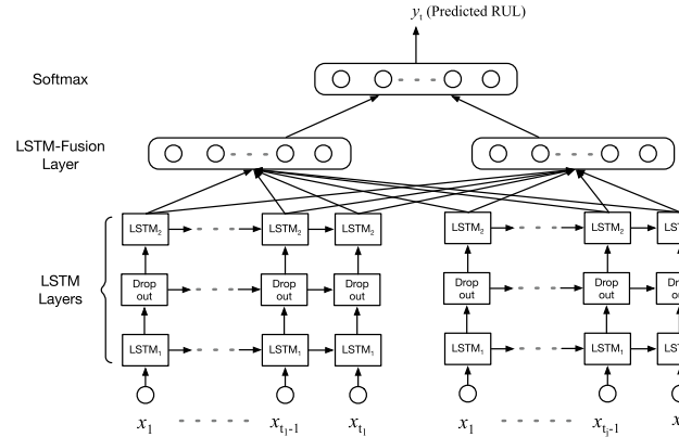
FIGURE 3. Proposed LSTM-Fusion network structure for RUL estimation.
