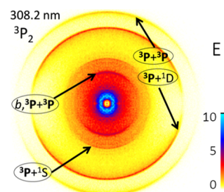
Figure 6. Raw S^+ image from S_2 recorded at 308.21 nm, the (2 + 1) REMPI wavelength for ionization of S^3P_2 atoms. The laser polarization direction E is parallel to the detector face and along the vertical axis of the figure. A color bar for conversion to signal intensity is given on the right side of the figure. For each labeled ring the detected atom is indicated by the bold typeface.
