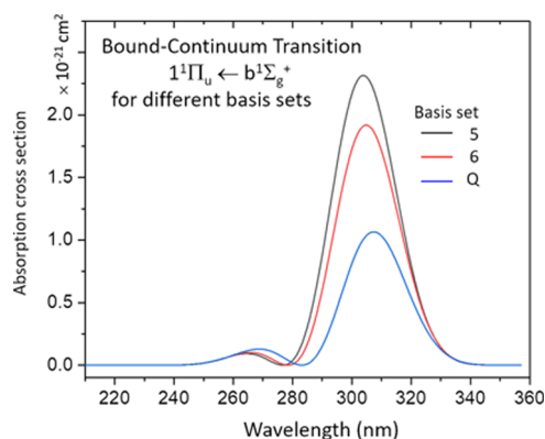
Figure 4. Absorption coefficient for the 1^1\Pi_u – b^1\Sigma_g^+ transition as a function of wavelength, shown for three different basis sets described in the text.
