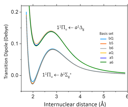
Figure 2. Transition dipole moment for the 1^1\Pi_u – b^1\Sigma_g^+ and 1^1\Pi_u – a^1\Delta_g transitions for three different basis sets described in the text.
