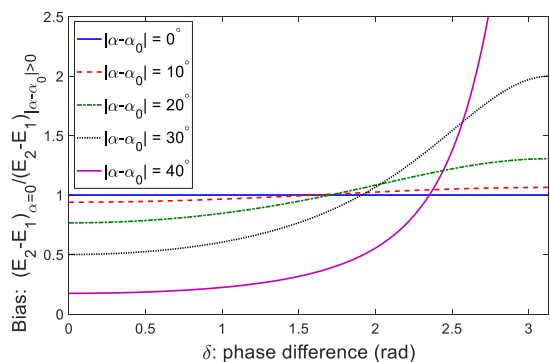
Fig. 12. Bias in E_2 - E_1 (fabric asymmetry) estimate when measurement system is not aligned with principal axis system. A bias > 1 indicates an overestimation of E_2 - E_1 due to evaluation at a non-principal angle and a bias < 1 indicates an underestimation.
