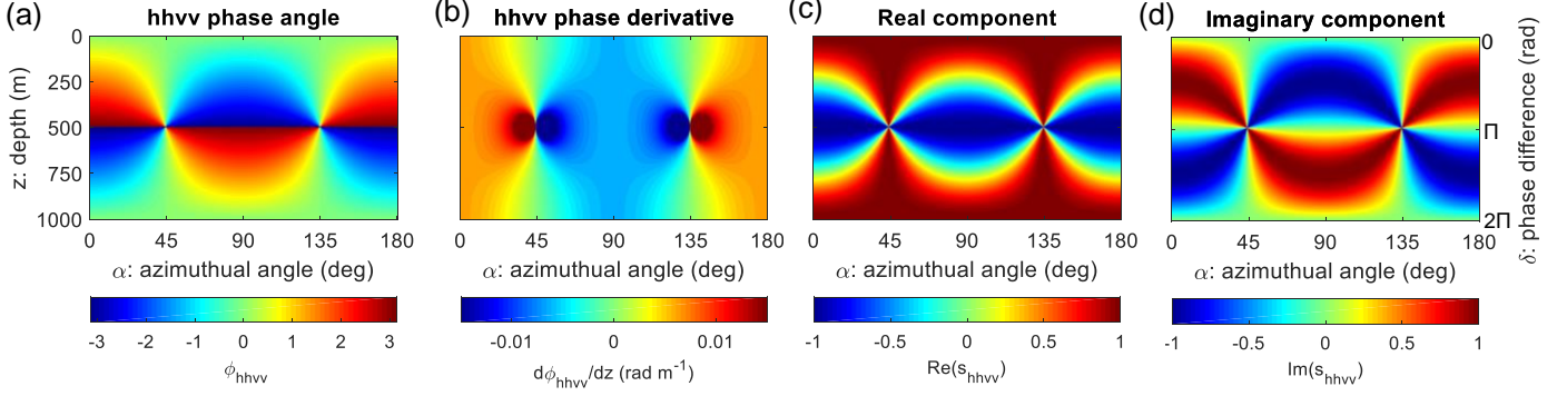
Fig. 2. Matrix backscatter model results for s_{hhvv} with isotropic scattering ( r = 1 ). (a) hhvv phase, \phi_{hhvv} = \arg(s_{hhvv}) . (b) Vertical hhvv phase gradient, d\phi_{hhvv}/dz . (c) Real component, \text{Re}(s_{hhvv}) , (d) Imaginary component, \text{Im}(s_{hhvv}) . The relationship between z and \delta assumes a two-way phase shift following (18) with a fixed fabric birefringence of \Delta\epsilon = 0.00354 and radar center frequency, f = 150 MHz. When \alpha = 0^\circ the v polarization is aligned with the greatest principal permittivity resulting in a positive hhvv phase gradient.
