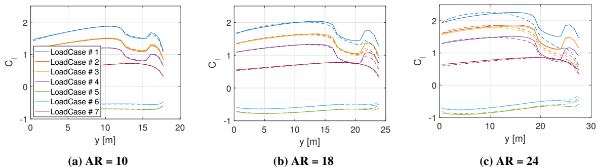
Fig. 13 Local lift coefficient along the wing for a) AR = 10 , b) AR = 18 and c) AR = 24 . Solid lines are linear and dashed lines are nonlinear.
