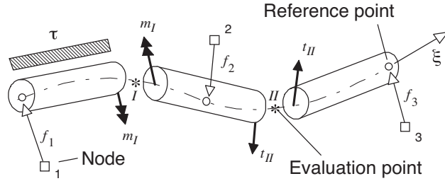
Fig. 3 Three node linear/nonlinear finite volume beam element
