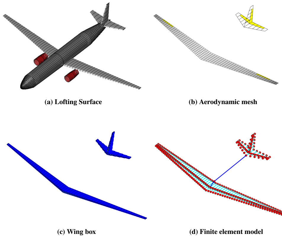
Fig. 6 Baseline Model
