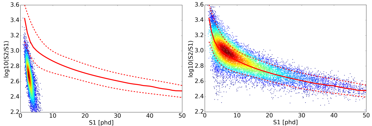
Figure 2.2.1: Calculated high-statistics probability distribution functions (PDFs) for ^8\text{B} (left panel) and atmospheric (right panel) coherent neutrino-nucleus scattering events. The solid curve is the centroid of the nuclear recoil band, and the dotted lines define a \pm 3\sigma band. These lines are defined for a spectrum flat in nuclear recoil energy. The recoils from ^8\text{B} on the left fall outside the band because the bulk of the PDF is under the threshold, and correlated fluctuations must occur for events to enter this plot. In 5,600 tonne-day of LZ exposure, we expect a mean of 7 and 0.5 NR events from these neutrino sources to meet selection requirements.
