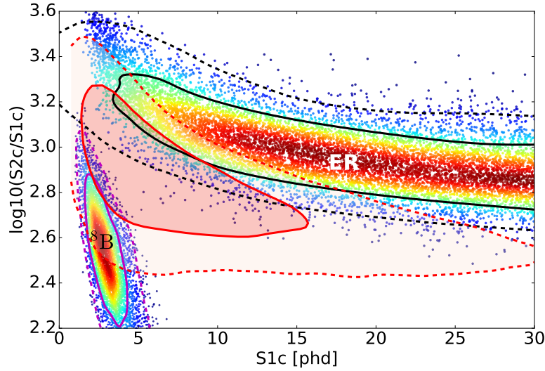
Figure 12.3.1: Simulations of the most prominent ER and NR (from ^8\text{B} ) backgrounds are plotted in the \log_{10}(S2c/S1c) - S1c plane. The statistics shown represent 5\times the expected ER background and 500\times the expected NR background in the nominal LZ exposure. The red tinted area shows the expectation for events from a 40\text{ GeV}/c^2 -mass WIMP, falling between the two background populations with the region enclosed by the solid(dashed) line representing the 1\sigma(2\sigma) band.
