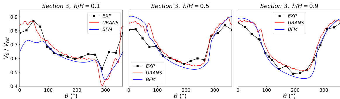
Figure 15. Azimuthal distribution of absolute tangential velocity in Section 3.
