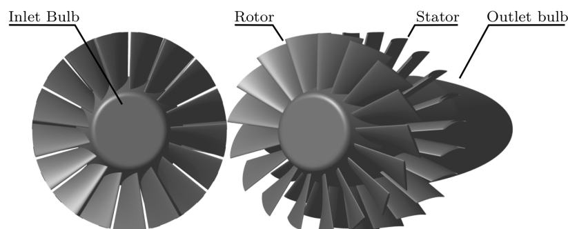
Figure 1. 3D view of the fan stage.
