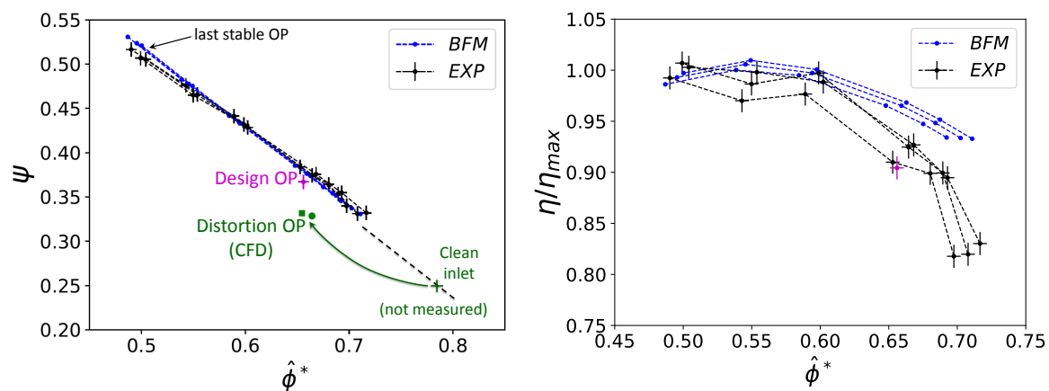
Figure 8. Global performance of the fan stage, clean inlet case, and distorted case.
