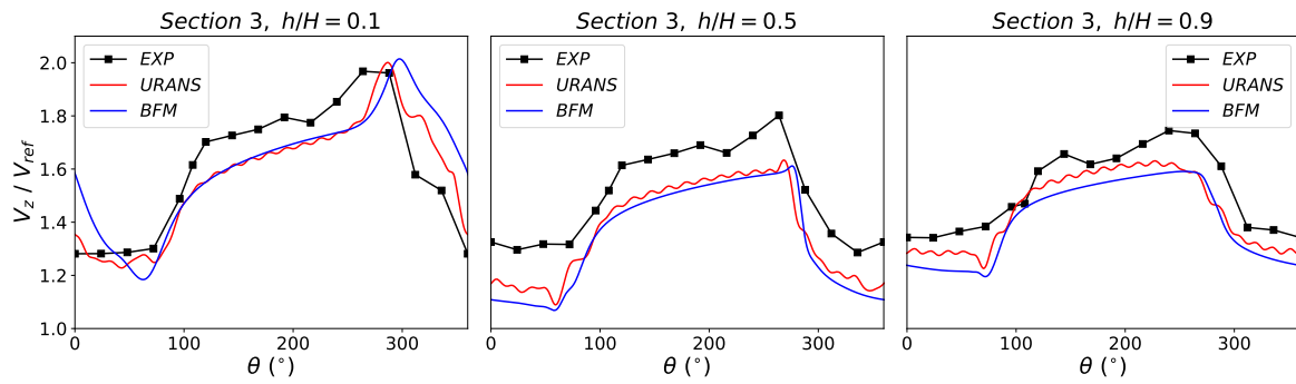
Figure 13. Azimuthal distribution of axial velocity in Section 3.
