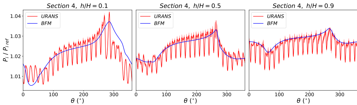
Figure 18. Azimuthal distribution of absolute total pressure in Section 4.
