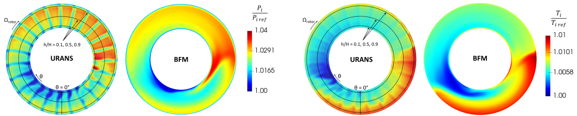
(a) Absolute total pressure field (b) Absolute total temperature field Figure 17. Comparison of URANS and BFM results in Section 4.
