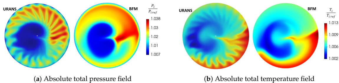
Figure 20. Comparison of URANS and BFM results in Section 5.
