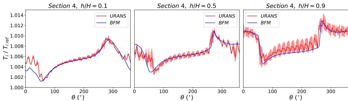
Figure 19. Azimuthal distribution of absolute total temperature in Section 4.
