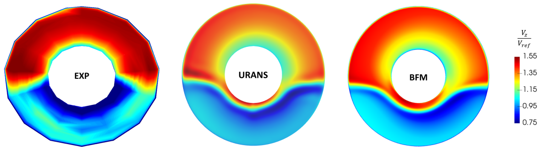
Figure 16. Axial velocity field in Section 2.
