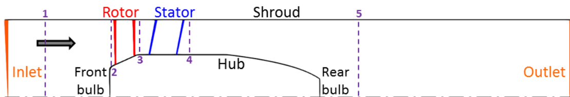
Figure 4. Meridional view of the computational domain.
