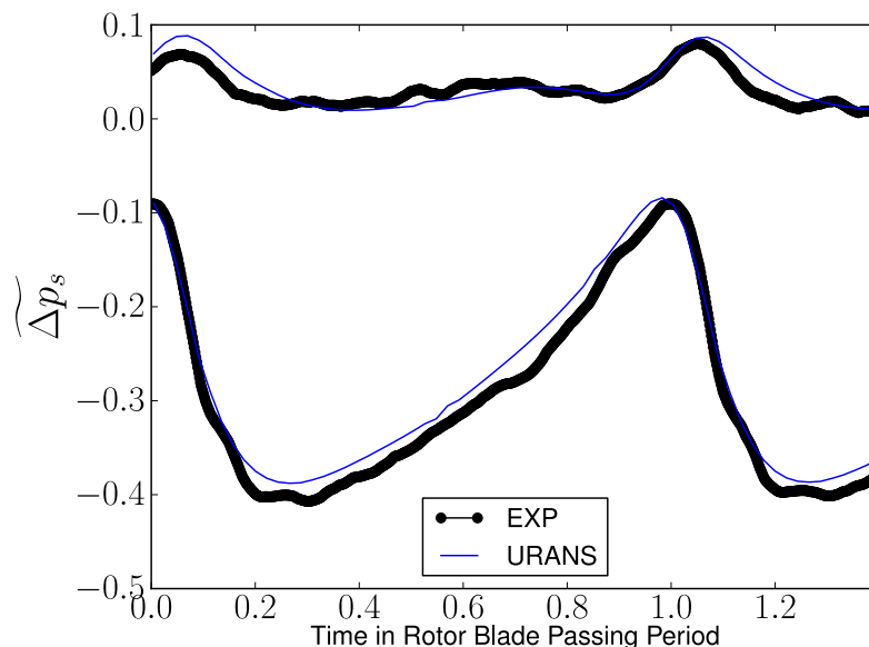
Figure 5. Pressure fluctuations at the rotor LE and TE at peak efficiency.
