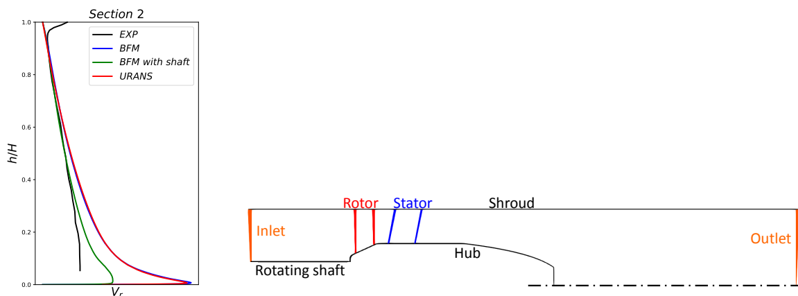
(a) Radial velocity profile at Rotor LE (b) Meridional view simulating the upstream shaft Figure 11. Influence of the shaft on the Rotor LE flow conditions.
