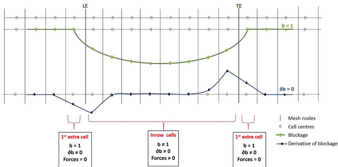
Figure 7. 1D representation of blockage and its derivative.
