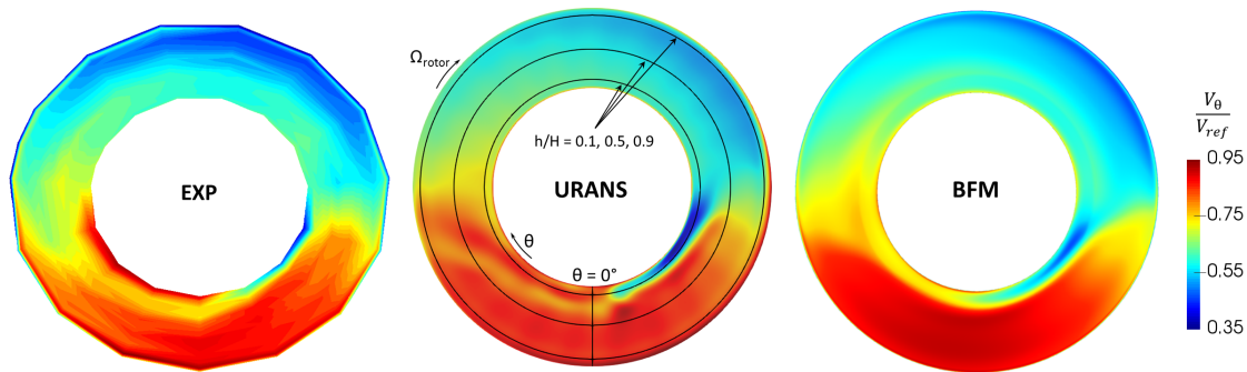
Figure 14. Absolute tangential velocity field in Section 3.
