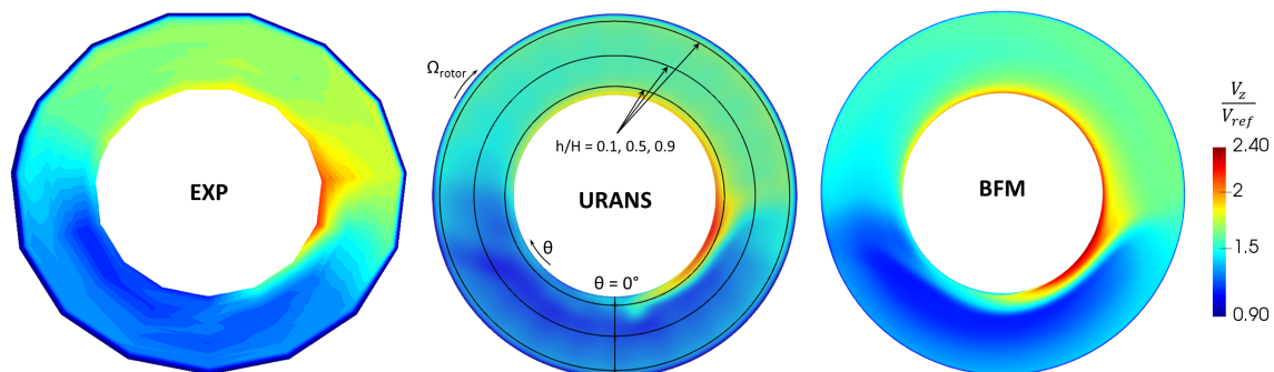
Figure 12. Axial velocity field in Section 3.
