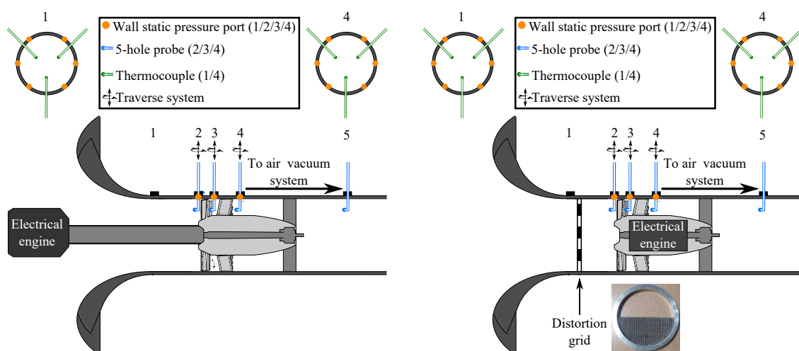
Figure 2. Schematic of the two experimental configurations, without/with distortion.
