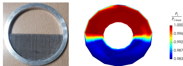
Figure 3. Distortion grid and measured total pressure pattern associated.
