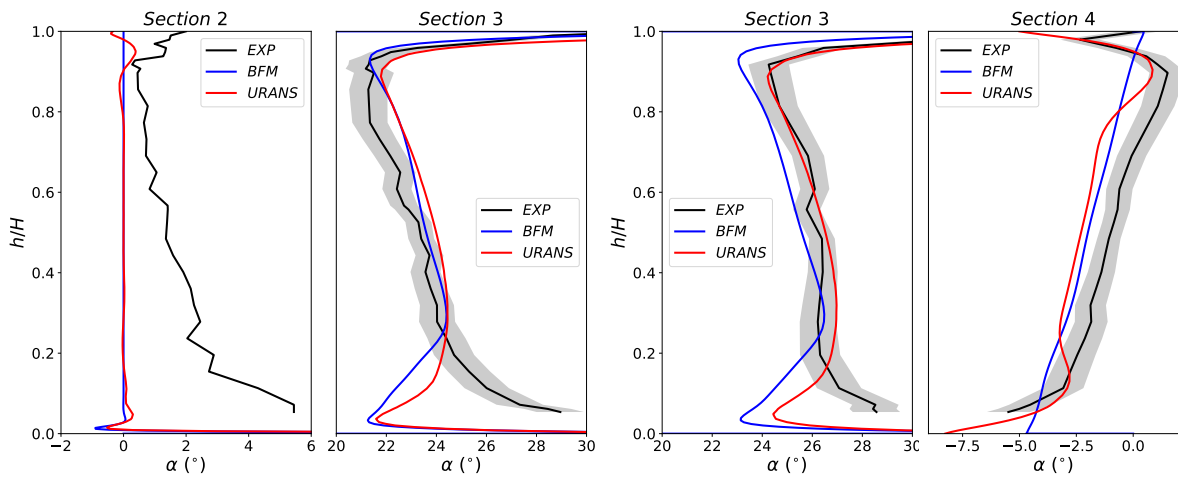
(a) At Rotor LE and TE (b) At Stator LE and TE Figure 10. Absolute flow angle radial profiles at design flow coefficient.
