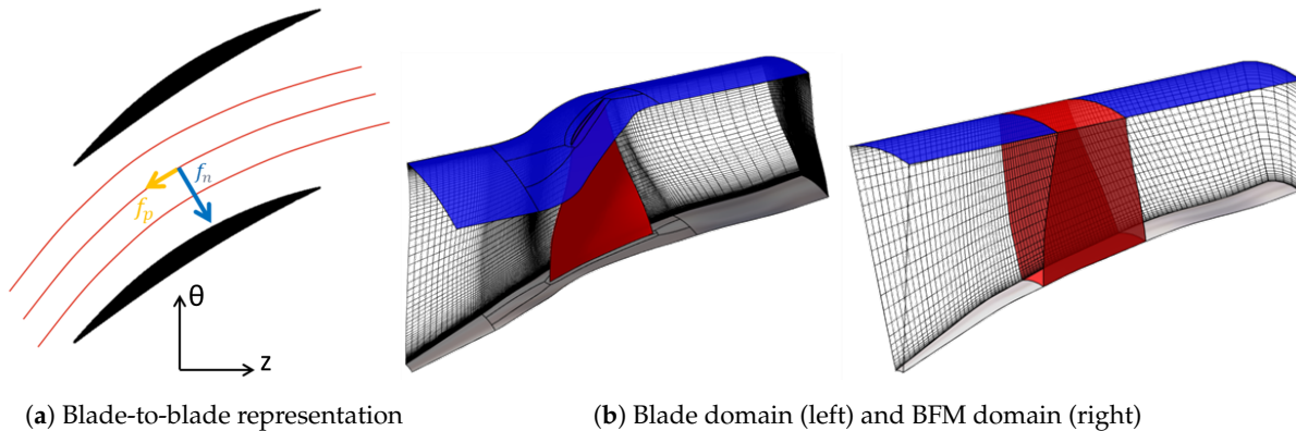
Figure 6. Illustration of the generic body forces methodology.
