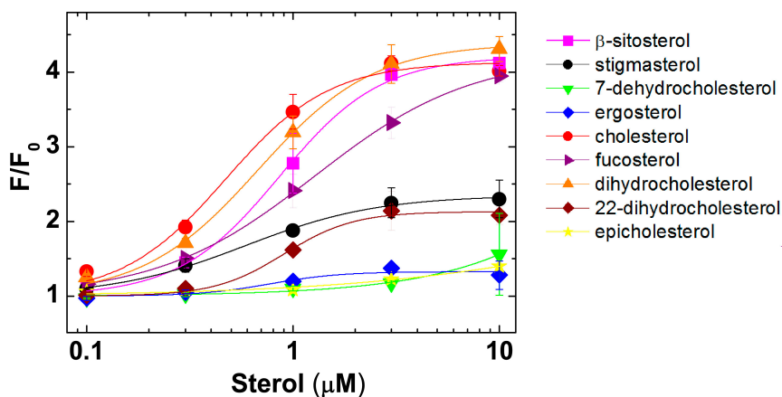
Figure 5. Binding of sterols to the PFO derivative containing the native undecapeptide (nPFO) [33]. Trp emission intensity for 0.1 \mu\text{M} nPFO was measured before ( F_0 ) and after ( F ) addition of the indicated amount of sterol. Each data point shows the average of at least two measurements and their range. The cholesterol concentration that produced half of the total Trp emission increase for nPFO was 0.5 \mu\text{M} .
