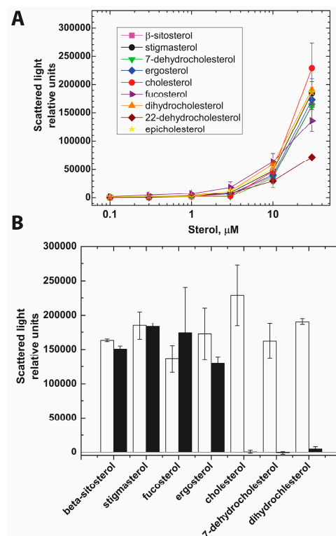
Figure 4. Sterol precipitated when added into aqueous buffer solution and they were differentially solubilized by mCD. (A) Scattered light at 500 nm of aqueous buffer solutions containing the indicated amount of sterols. Sterols were added from ethanolic solutions incrementally and incubated 5 min at 37 °C before each measurement; (B) mCD (final concentration 3 mM) was added into solutions containing 30 \mu\text{M} sterols and the right angle light scatter measured after 5 min incubation at 37 °C. The bars represent the average of at least two measurements and the error bars correspond to the range. White bars and black bars represent the scattered light before and after incubation with mCD, respectively.
