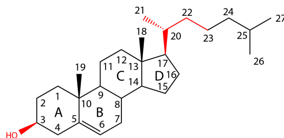
Figure 3. Chemical structure of cholesterol showing the individual rings (A)–(D) and numbered carbon atoms. Elements identified as critical for the interaction with CDCs are indicated in red.
