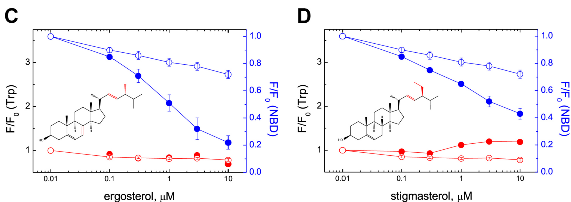
Figure 6. Sterol binding to D4 paralleled the conformational change in D3. rPFO V322C-NBD (0.1 \mu\text{M} ) was titrated with (A) 7-dehydrocholesterol, (B) \beta -sitosterol, (C) ergosterol, (D) stigmasterol, and the Trp emission intensity and NBD emission intensity were determined in the same sample at each sterol concentration. Open symbols correspond to a parallel experiment where an identical volume of ethanol was added (no-sterol control). Trp emission data are shown in red, whereas NBD emission data are shown in blue. The average of at least two independent measurements and their range are shown. As a reference, the cholesterol concentration that produced half of the total NBD emission decrease for rPFO V322C-NBD was 0.8 \mu\text{M} [33].
