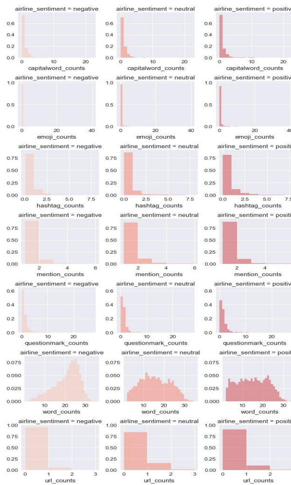
Figure 7: Distribution of Text Variables.
