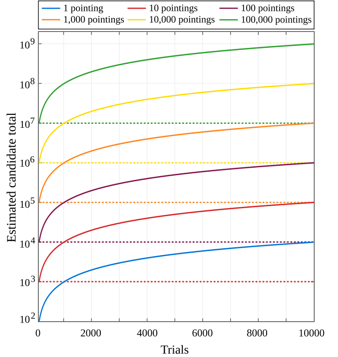
Figure 3. Candidate numbers predicted by Equation 4 (using n_\sigma = 7 and n_\sigma^{\max} = 100 ), varied according to the total number of survey pointings for a single beam receiver. Coloured dashed lines indicate the total number of candidates returned when using a conservative C = 100 cut. The corresponding solid colour lines indicate the total number of candidates returned when the cut is discarded. The solid lines are truncated such that they begin where C = 100 to avoid overlapping lines complicating the plot.
