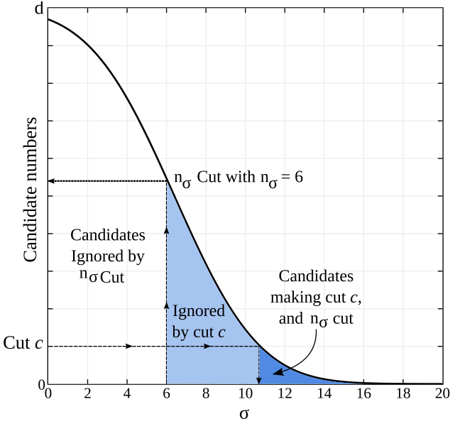
Figure 2. Diagram of 1 - \text{CDF} of Equation 1, showing the relationship between n\sigma and constant cuts. This illustrates their impact on the number of noise candidates making it through to the candidate selection stage.
