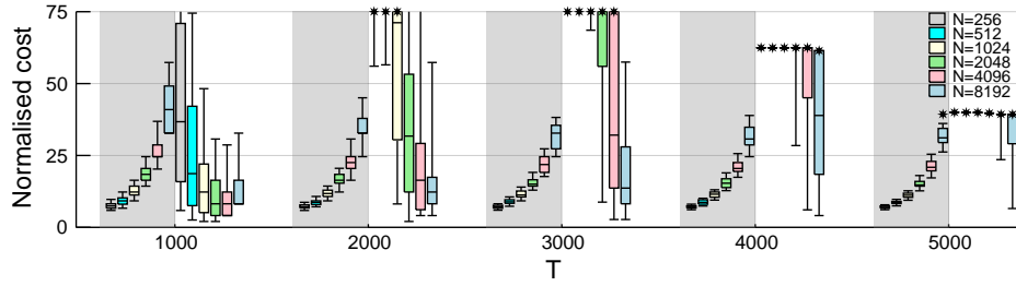
Fig 3: Normalised cost of coupling for the simple homogeneous model for 100 replications of BS and AS, the former on shaded background. The stars indicate cases where at least one replication failed to couple before hitting the maximum total cost. Since the normalised cost of coupling is plotted, the actual differences in computational cost are obtained by scaling by T^2 .
