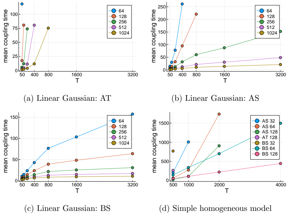
Fig 1: Mean coupling times associated with ancestor tracing (AT), ancestor sampling (AS) and backward sampling (BS). For (d), the lines are coloured according to the type of algorithm and the number of particles N .
