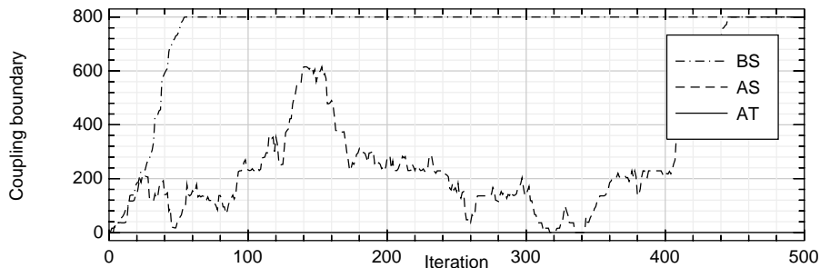
Fig 2: One realisation of coupling boundaries with T = 800 and N = 64 .
