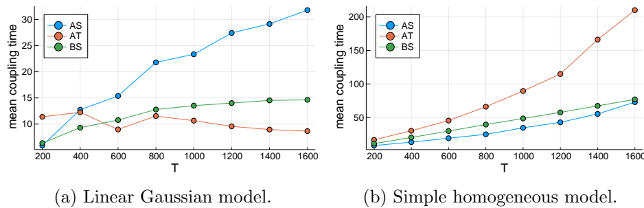
Fig 4: Mean coupling times associated with ancestor tracing (AT), ancestor sampling (AS) and backward sampling (BS). For the linear Gaussian model, N = 2.56T for AT whereas N = 512 for AS and BS. For the simple homogeneous model, N = 0.64T for AT and AS, whereas N = 128 for BS.
