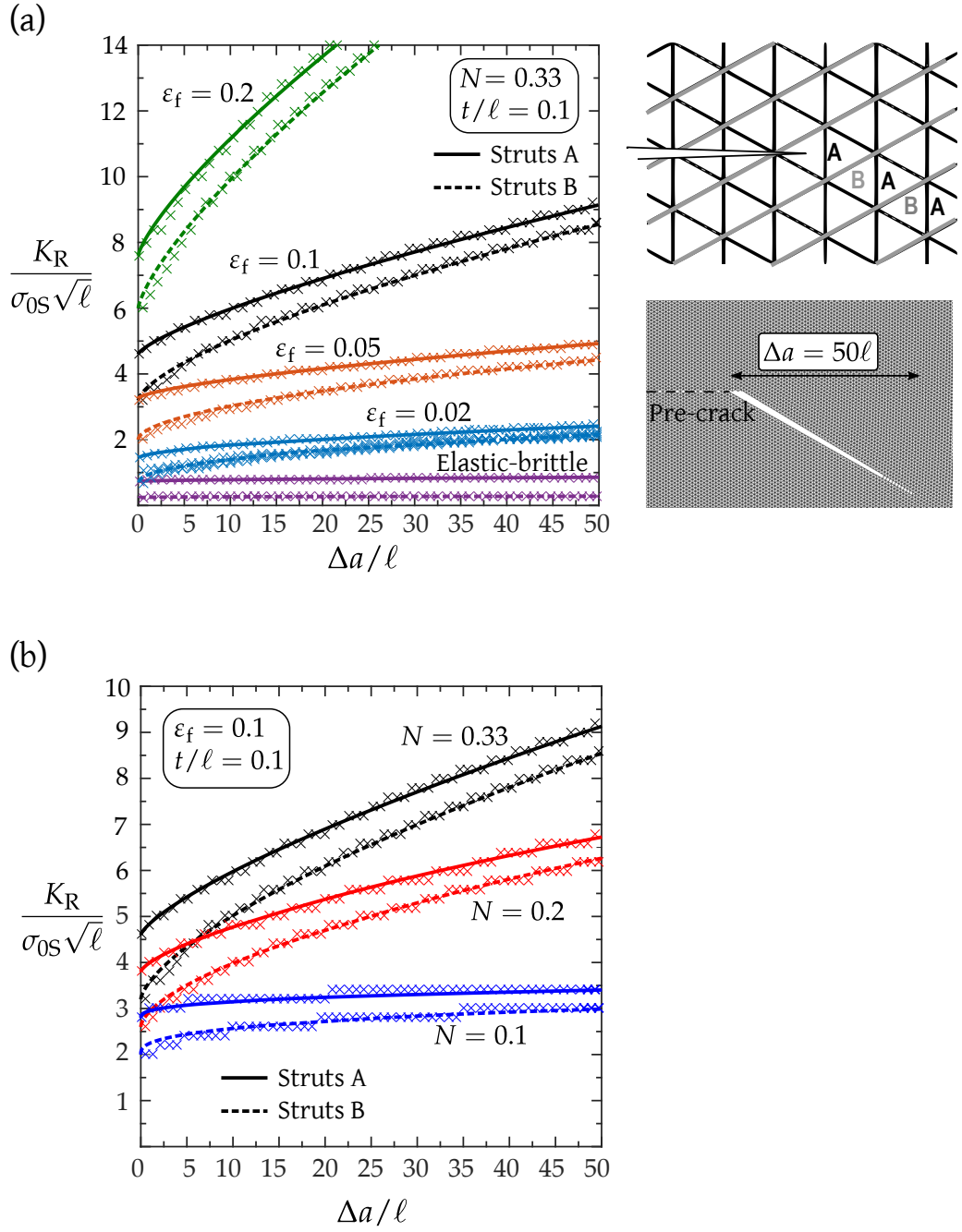
Fig. 8: Mode II crack growth resistance of an elastoplastic triangular lattice : (a) as a function of strut ductility \varepsilon_f for a choice of N = 0.33 , and (b) as a function of the strain-hardening exponent N for a choice of \varepsilon_f = 0.1 . In all cases, \varepsilon_{0S} = 0.001 , t/\ell = 0.1 , and \bar{\Gamma} = 5 . Inset of (a) shows predicted crack path at \Delta a = 50\ell for crack growth under remote mode II loading.
