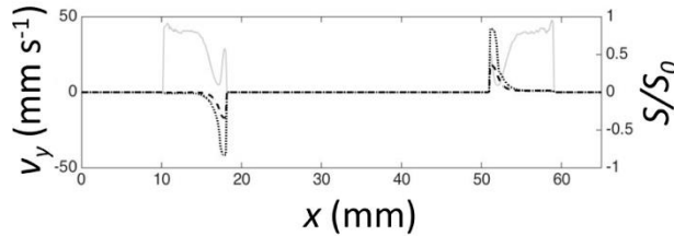
FIG. 2. Velocity and signal magnitude profiles across the gap are shown for two different inner wall velocities, U = 17 \text{mm s}^{-1} (dashed) and U = 41 \text{mm s}^{-1} (dotted). The normalized 1D signal intensity profile for U = 41 \text{mm s}^{-1} is shown in grey. For both shear rates the velocity profile decays to approximately zero well before the stationary, outer wall.
