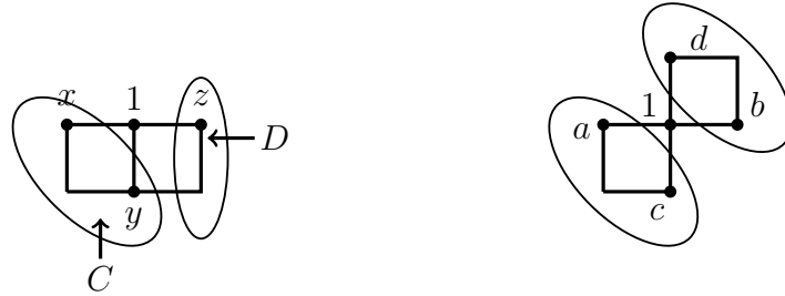
Figure 2.8: Two subcases when 1 belongs to exactly two squares
