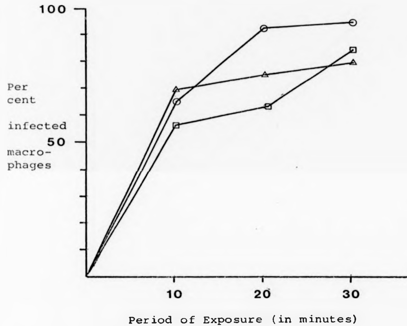
Fig. 2 Relationship of time of exposure to and volume of parasite suspension to macrophage parasitization. Percentage of infected cells as a function of time. Macrophages were exposed to parasites at a ratio of five parasites per macrophage suspended in 0.25 ml ( \Delta ), 0.5 ml ( \circ ) and 1 ml ( \square ). Each point on the graph represents the average of duplicate assays.
