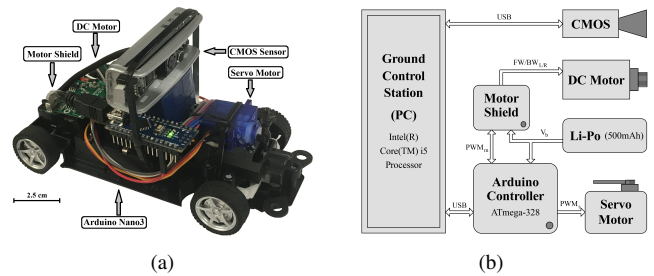
Fig. 7. Robotic platform. (a) Assembled platform used for real-time real-world experimentation. (b) Simplified circuit connection depicting every component involving a basic 2-Megapixel CMOS sensor, an Atmel ATmega328 8-bit AVR micro-controller, basic servos and motors, and a ground control station PC (Intel Core i5-6500, 8GB RAM).
