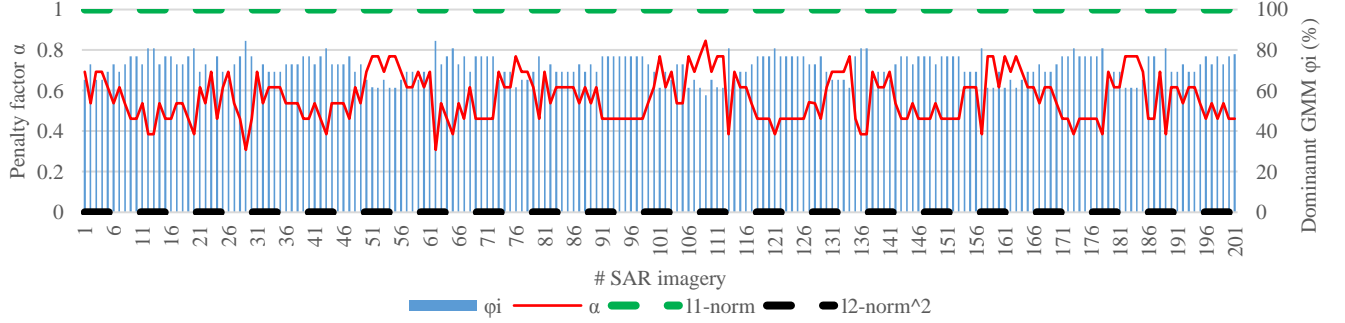
Fig. 2. Dependency of penalty factor a with the dominant GMM distribution \phi_i
