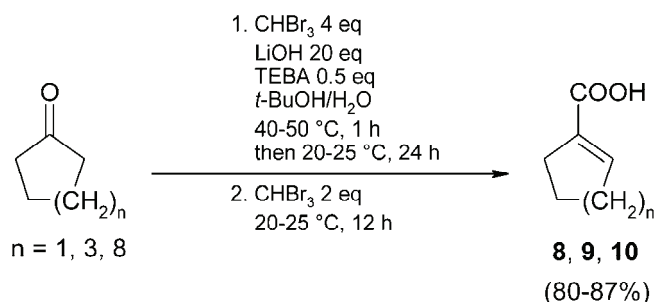
Scheme 2. Optimized one-pot reaction of cyclic ketones with bromoform.
