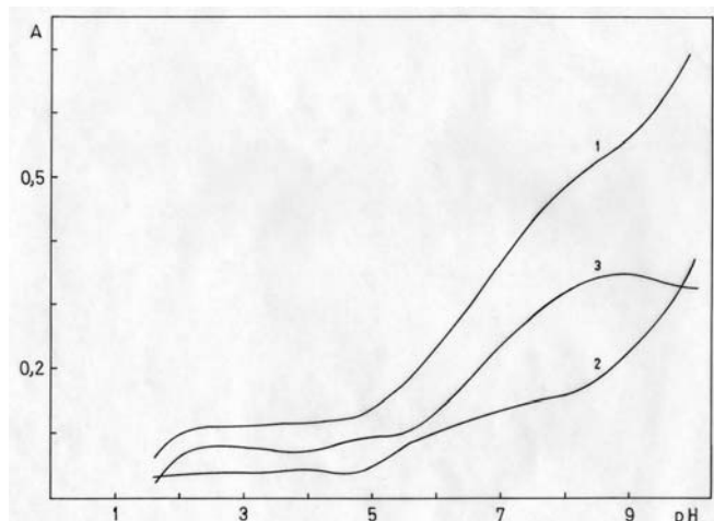
Slika 4. Zavisnost apsorbancije od pH: kriva 1: smeša 5,0 \cdot 10^{-5} \text{ mol dm}^{-3} \text{ K}_2\text{TiO}(\text{C}_2\text{O}_4)_2 i 1,0 \cdot 10^{-3} \text{ mol dm}^{-3} morina kriva 2: 1,0 \cdot 10^{-3} \text{ mol dm}^{-3} morin kriva 3: \Delta A = f(\text{pH}) Slepa proba 50% V/V etanol, \lambda = 480 \text{ nm} .
