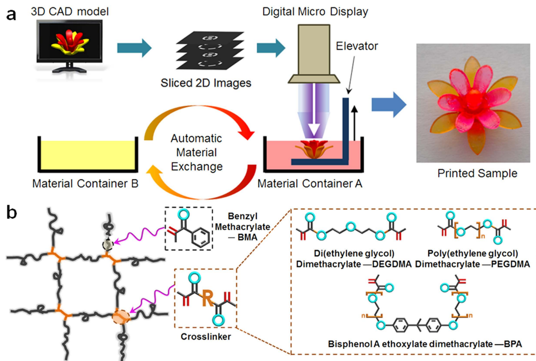
Figure 1. Schematics of multimaterial additive manufacture system. (a) A workflow illustrates the process of fabricating a multimaterial structure based on P \mu SL (b) Photo-curable shape memory polymer network is constructed by mono-functional monomer, Benzyl methacrylate (BMA) as linear chain builder (LCB), and multi-functional oligomers, Poly (ethylene glycol) dimethacrylate (PEGDMA), Bisphenol A ethoxylate dimethacrylate (BPA), and Di(ethylene glycol) dimethacrylate (DEGDMA) as crosslinkers.
