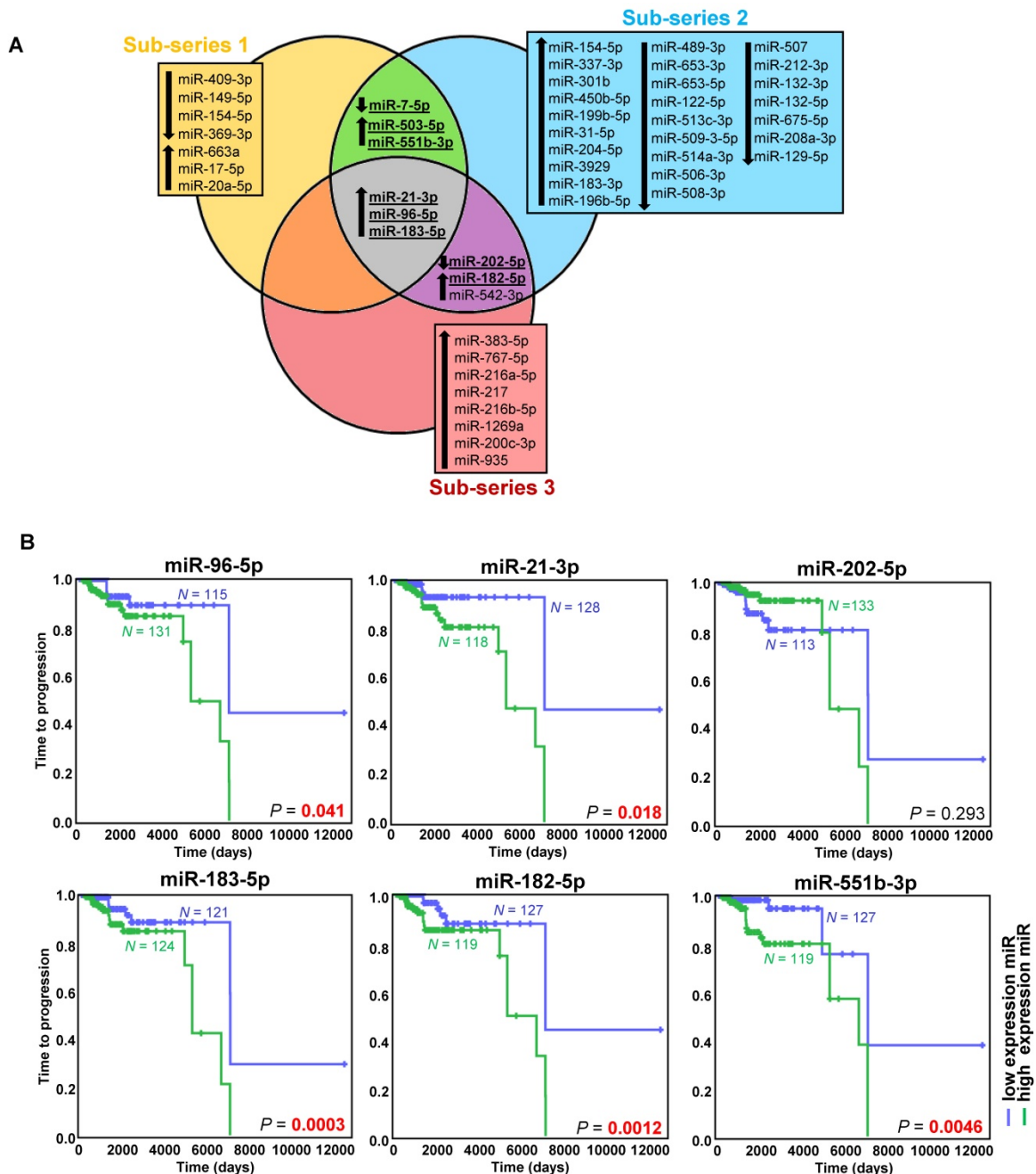
Figure 1. miRNAs associated with metastatic behavior. (A) Venn diagram of differentially expressed miRNAs ( FDR < 0.05 , |\log_2 \text{fold change}| \geq 0.75 ) in the different sub-series of the discovery series ( n=443 ). Downregulated miRNAs are indicated with a downward pointing arrow, and upregulated miRNAs are indicated with an upward pointing arrow. miRNAs selected for validation are shown in bold and are underlined. (B) Kaplan-Meier plots of time to progression (time between the first PPGL diagnosis and the first documented metastases) of patients according to the expression level of the indicated miRNA in tumor tissue. High expression (above the median expression level of the whole group) of the miRNA is represented in blue and low expression (below the median level) in green ( n=246 patients from the discovery and validation series, either presenting metachronous metastases — presented \geq one year after diagnosis —, or with more than one-year follow-up — median follow-up time=1290 days). Patients without evidence of metastases were censored at the date of the last follow-up. P -values were calculated with a log-rank test. N : number of patients.
