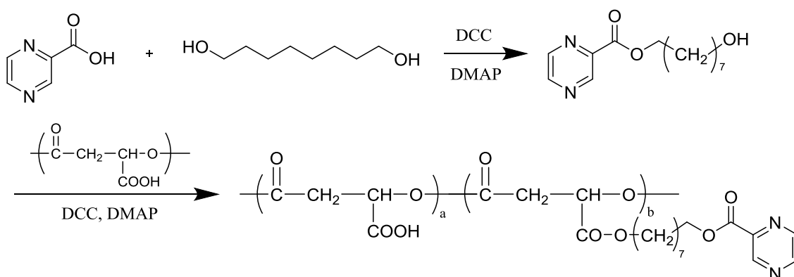
Fig. 1: Synthesis route for pyrazinoic acid ester conjugate (PMA:OctPA).
