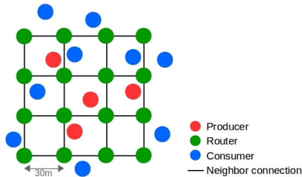
Figure 4: Topology example
