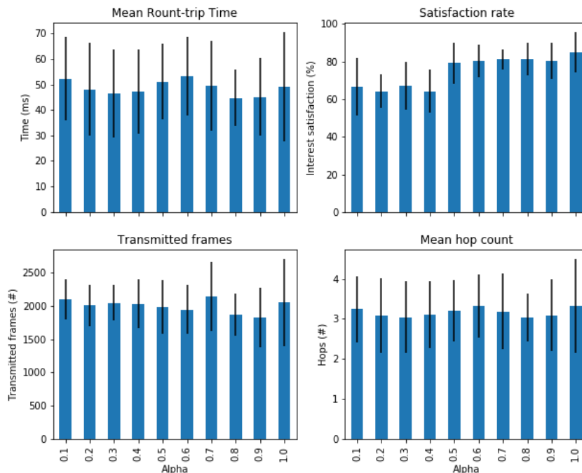
Figure 5: Impact of the learning rate
