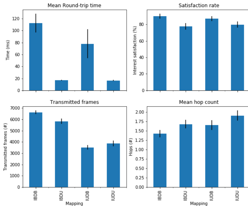
Figure 2: NDN-MAC mapping simulation results
