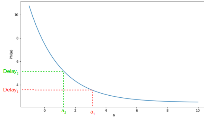
Figure 3: Delay function example
