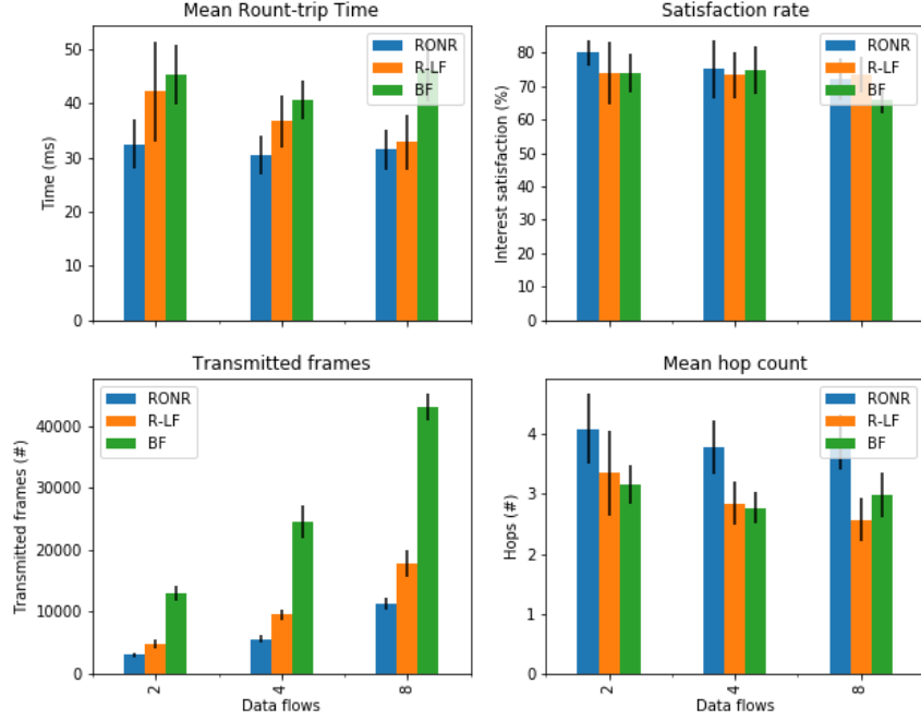
Figure 7: Multiple dataflows scenario results
