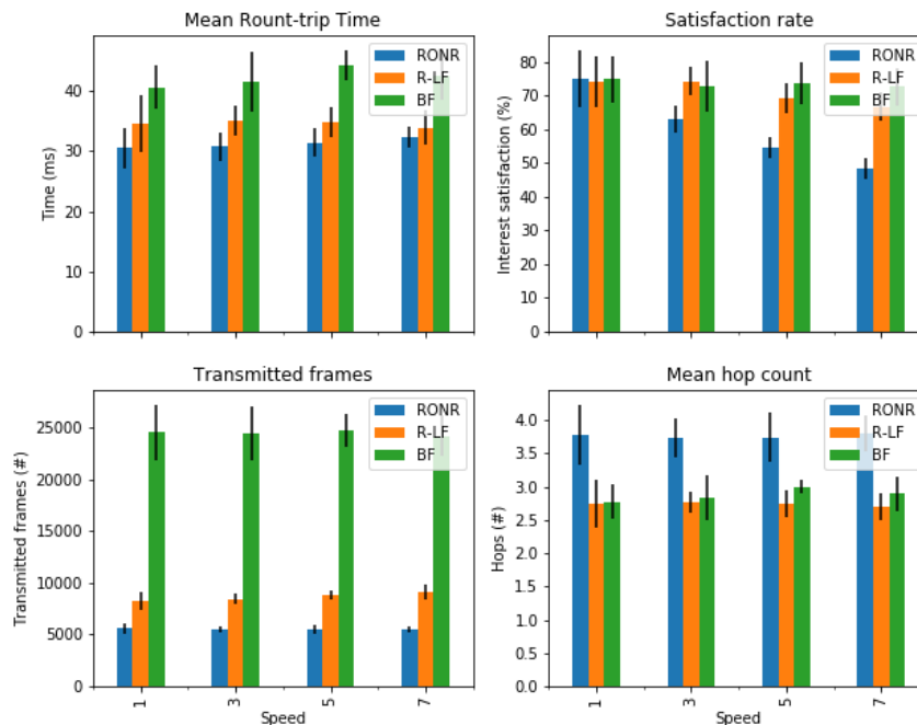
Figure 9: Producers speed scenario results
