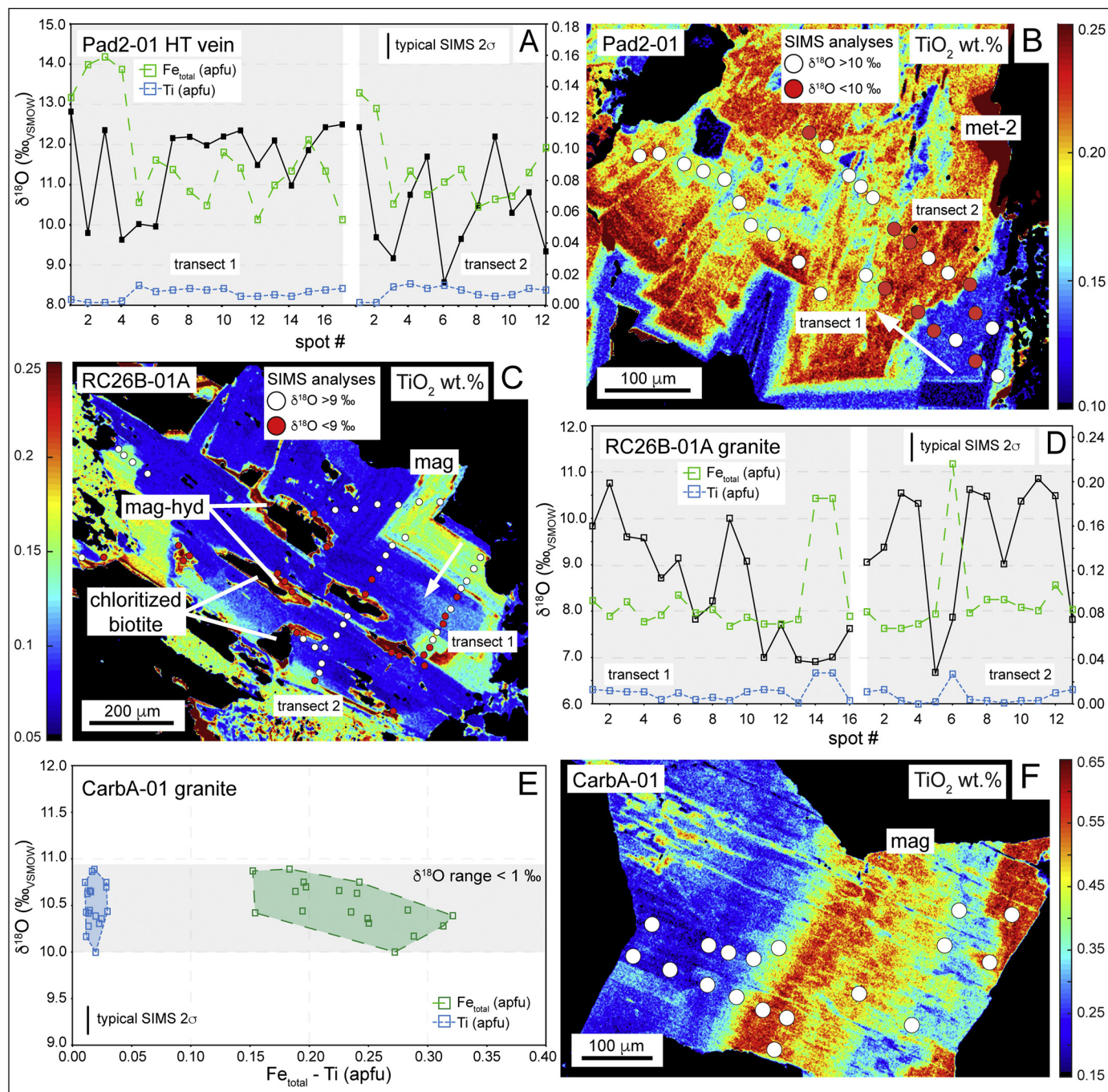
Fig. 6. Microscale \delta^{18}\text{O} variability of white mica versus chemistry and texture. A–B – chemically variably white mica met-2 in HT vein sample Pad2-01; C–D – primary granitic white mica with included chloritized biotite surrounded by altered areas in sample RC26B-01A; E–F – primary granitic white mica in sample CarbA-01. EPMA elemental maps in B, C, F depict zonation in \text{TiO}_2 (wt%). Spots on EPMA maps depict the location of the SIMS analyses.
