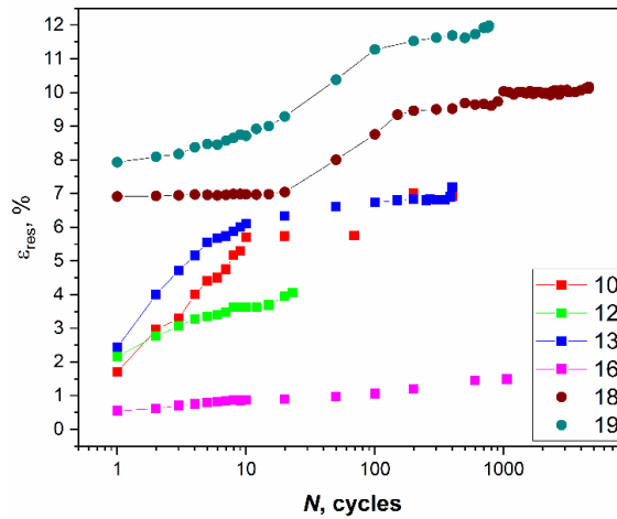
Fig. 2. Dependences of the residual strain – a) and strain range –b) on the number of loading cycles. \Delta\sigma = 492 MPa (16), 539 MPa (13), 580 MPa (10), 727 MPa (12) at stress ratio R = 0 , \Delta\sigma = 243 MPa (18), 305 MPa (19) at R = 0.5 .
