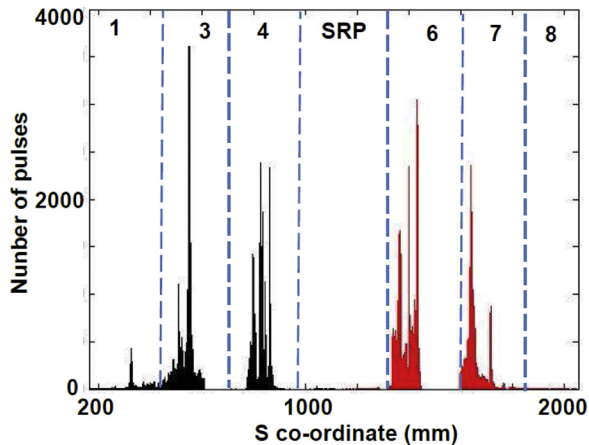
Fig. 14. Histogram showing the distribution of strike point positions in the divertor during the MkII-SRP operations 2001–4. The X-axis is the s co-ordinate: the changes from Tiles 1-3-4-5-6-7-8 occur at approximately 0.43, 0.7, 0.95, 1.32, 1.55 and 1.81 m.
