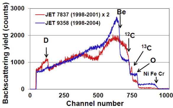
Fig. 33. RBS spectra from the upper part of the front face of Tile 3 for tiles removed in 2001 and in 2004. The arrows indicate the high energy edge of the feature characteristic of that element.
