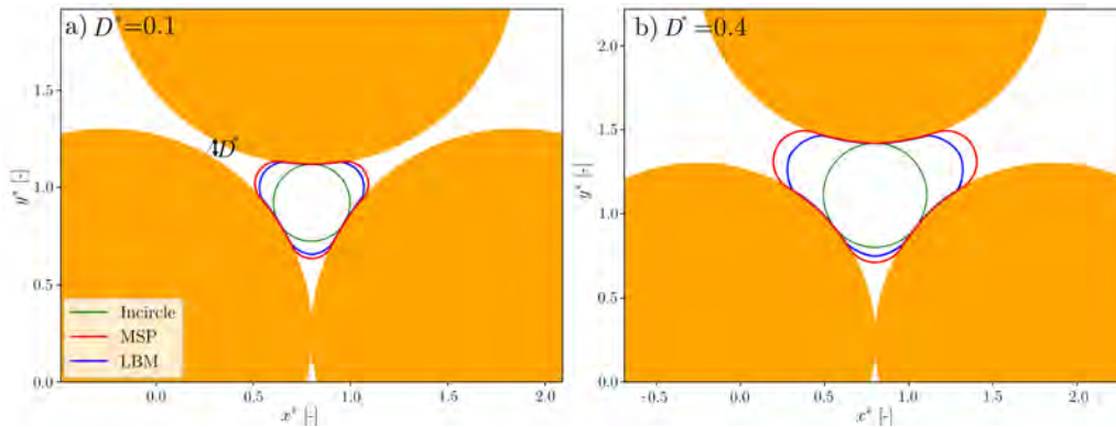
Figure 5.12: Overlapped MS-P, Incircle and LBM profiles when one of the grains is moved away from the other two while the rest remain in contact. a) D^* = 0.1 and p_{c,LB}^{*,e} = 12.2 . b) D^* = 0.4 and p_{c,LB}^{*,e} = 6.6 .
