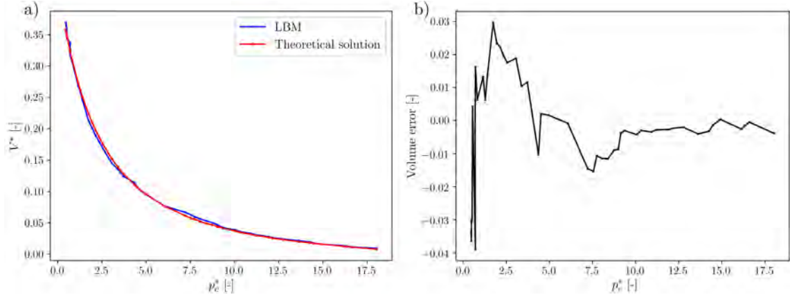
Figure 2.18: a) Volume versus capillary pressure for a pendular bridge from a LBM simulation and the numerical solution of Laplace-Young equation. b) The relative error is the difference between the simulated volume and the theoretical volume normalized as V^* = V/R^3 .
