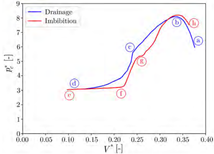
Figure 5.21: p_c^* - V^* relationship at a pore throat under a drainage-imbibition cycle.
