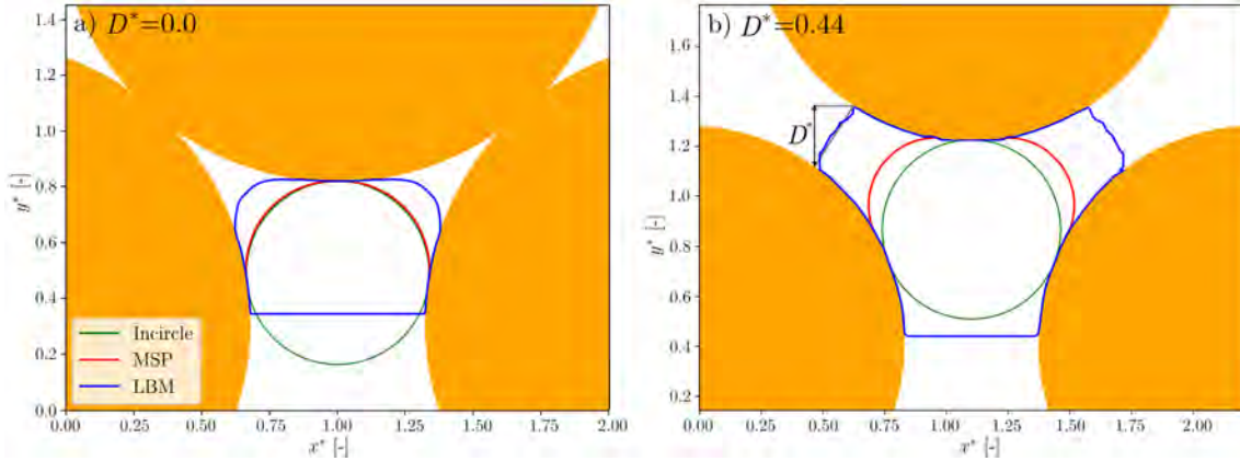
Figure 5.14: Overlapped MS-P, Incircle and LBM profiles when one of the grains is moved away from the other two. The rest of the spheres are not in contact. a) D^* = 0.0 and p_{c, LB}^{*,e} = 7.4 . b) D^* = 0.44 and p_{c, LB}^{*,e} = 4.2 .
