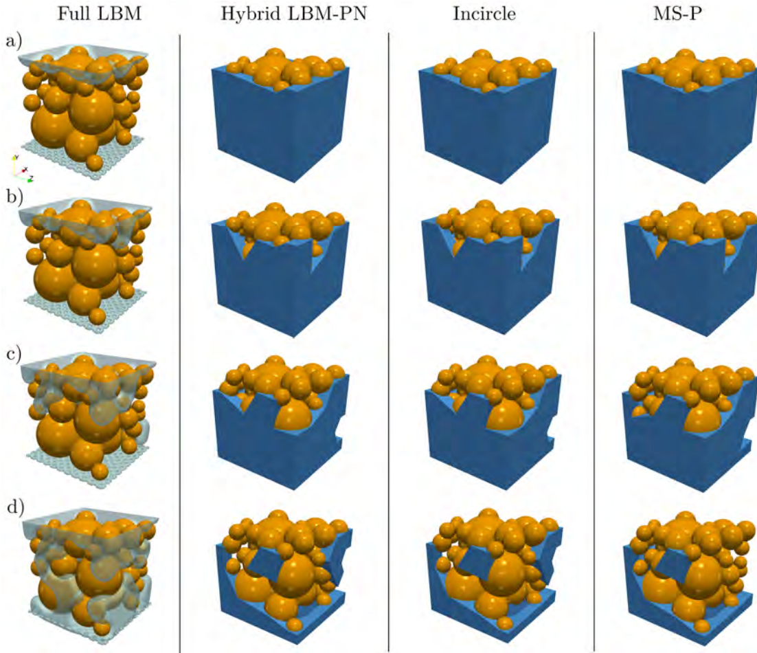
Figure 6.14: Comparison of the invasion path between the full LBM simulation, Hybrid, MS-P and Incircle methods. Front view. a) p_c^* = 2.4 , b) p_c^* = 3.3 , c) p_c^* = 4.2 and d) p_c^* = 5.3 .
