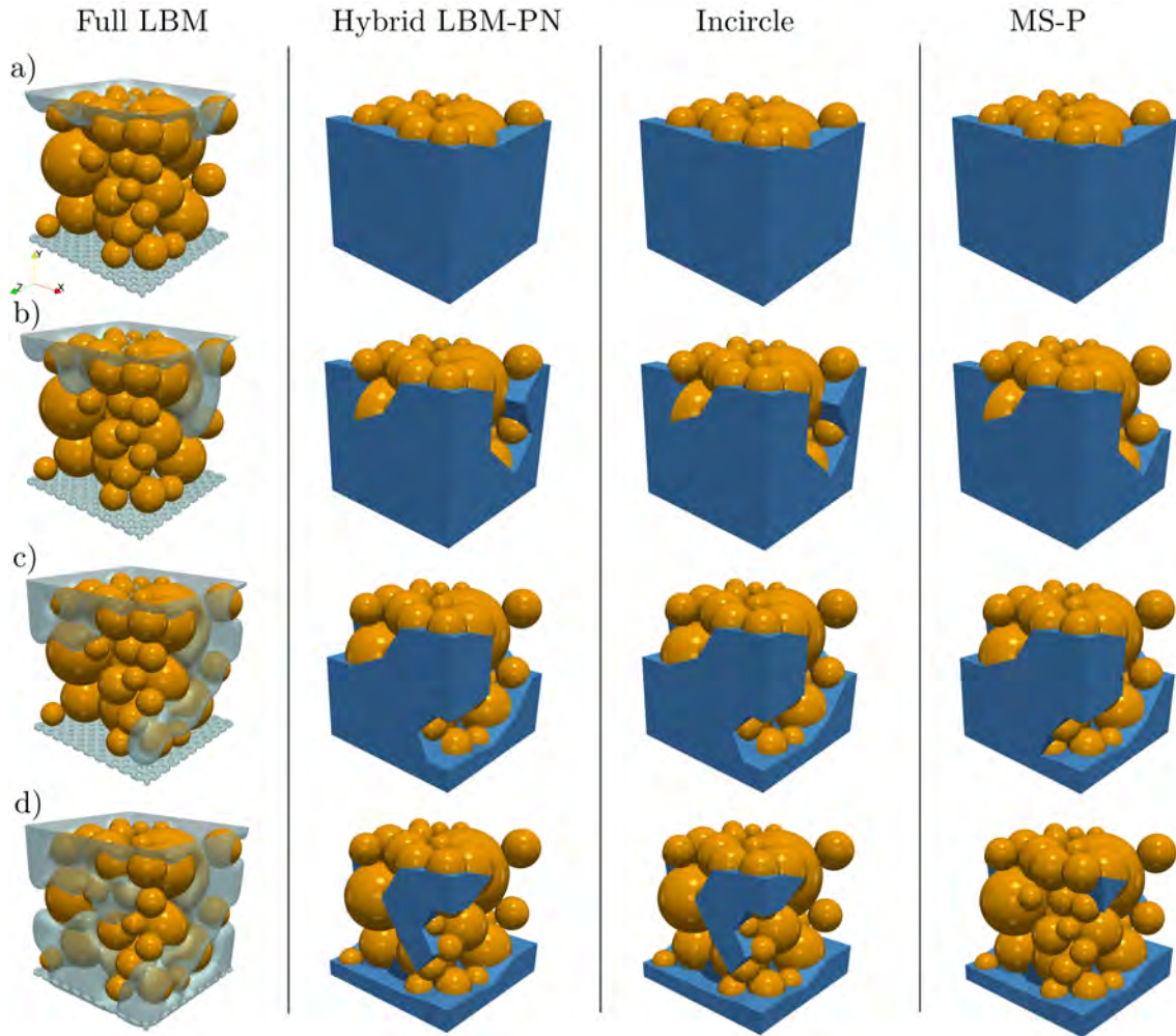
Figure 6.13: Comparison of the invasion path between the full LBM simulation, Hybrid, MS-P and Incircle methods. Back view. a) p_c^* = 2.4 , b) p_c^* = 3.3 , c) p_c^* = 4.2 and d) p_c^* = 5.3 .
