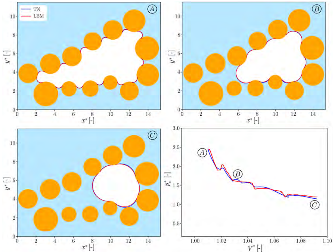
Figure 4.7: Comparison of interface position between LBM and TN models. The capillary pressure is deliberately reduced to force the imbibition of the macro-pore. The menisci begin merging with other menisci as they increase the radii. Gradually, the system is getting more saturated. Various liquid contents are displayed: \textcircled{A} V^* = 1.01 , \textcircled{B} V^* = 1.03 and \textcircled{C} V^* = 1.09 .
