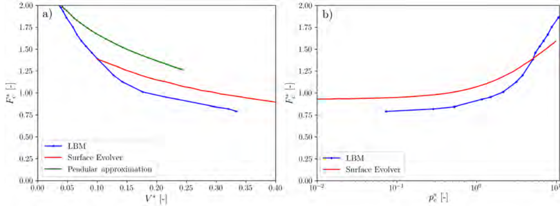
Figure 3.14: a) Liquid volume vs. capillary for spheres in contact under drainage conditions. Comparison between pendular approximation, LBM and the results for SE obtained in Wang et al. (2017). b) Evolution of capillary force with the suction. Comparison between LBM and the results for SE obtained in Wang et al. (2017) in logarithmic scale
