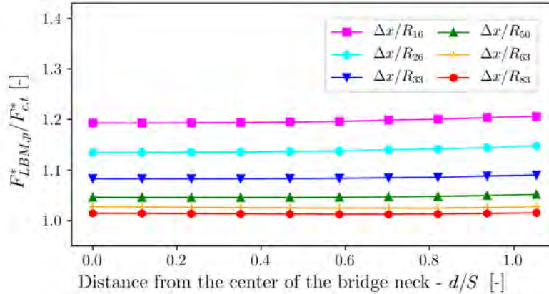
Figure 3.7: Capillary forces error in function of mesh size and distance ( d ) from the center of the bridge neck. All the simulations correspond to a capillary pressure of p_c^* = 0.4 and a separation distance of S^* = 0.2 between the spheres. Force is evaluated with Eq. 3.1 after computing the radius neck for each LBM simulation.
