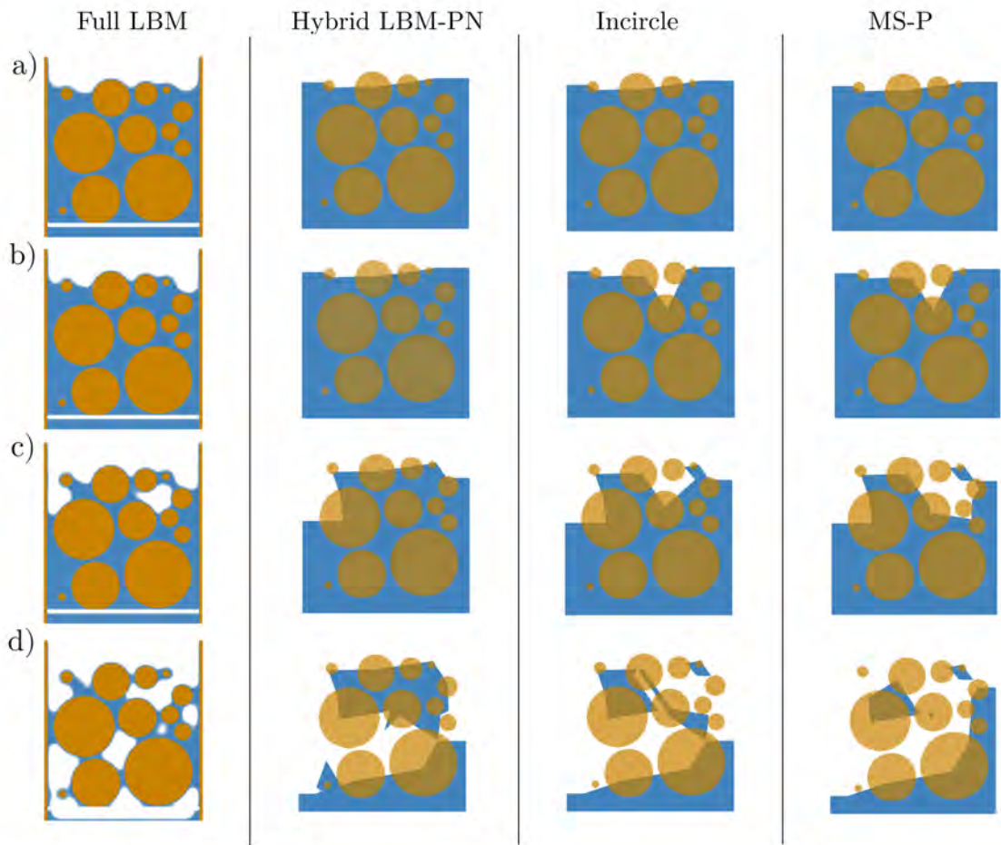
Figure 6.16: Comparison of the invasion path for plane A (see figure 6.15). a) p_c^* = 2.4 , b) p_c^* = 3.3 , c) p_c^* = 4.2 and d) p_c^* = 5.3 .
