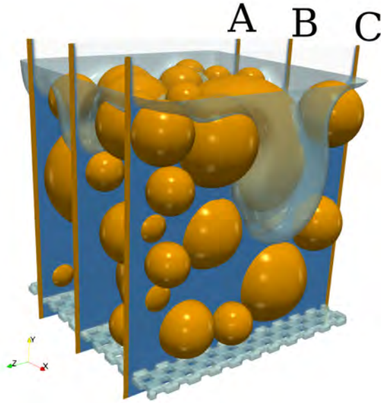
Figure 6.15: Vertical slices of the granular assembly.
