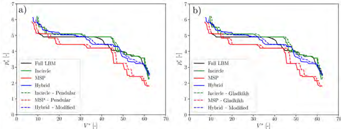
Figure 6.7: Primary drainage curves obtained with different methods including meniscus. MS-P and Incircle account for the extra volume by means of the Pendular (a) and Gladkikh approximation (b).
