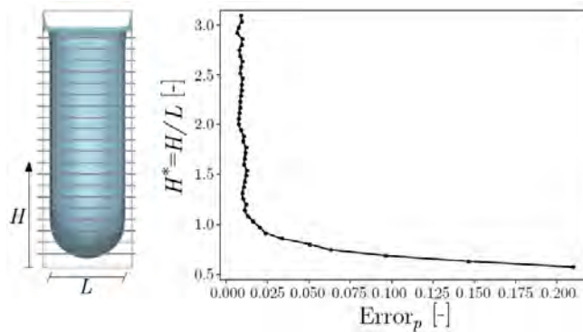
Figure 2.16: Evolution of the error on pressure by applying MS-P versus distance from the main meniscus. Drainage of a square cylinder.
