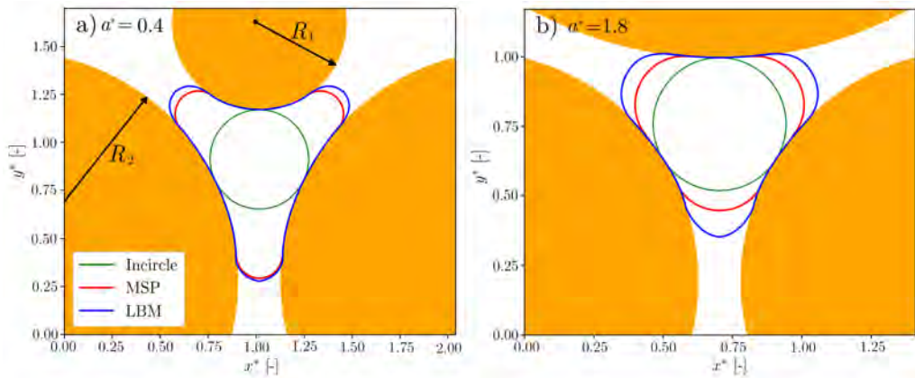
Figure 5.16: Overlapped MS-P, Incircle and LBM profiles for different radius ratios. a) a^* = 0.4 and p_{c,LB}^{*,e} = 6.0 . b) a^* = 1.8 and p_{c,LB}^{*,e} = 8.2 .
