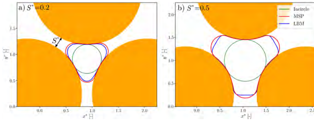
Figure 5.9: Overlapped MS-P, Incircle and LBM profiles when the 3 spherical bodies are moved away from each other. a) S^* = 0.2 and p_{c, LB}^{e,*} = 7.5 . b) S^* = 0.5 and p_{c, LB}^{*,e} = 4.2 .
