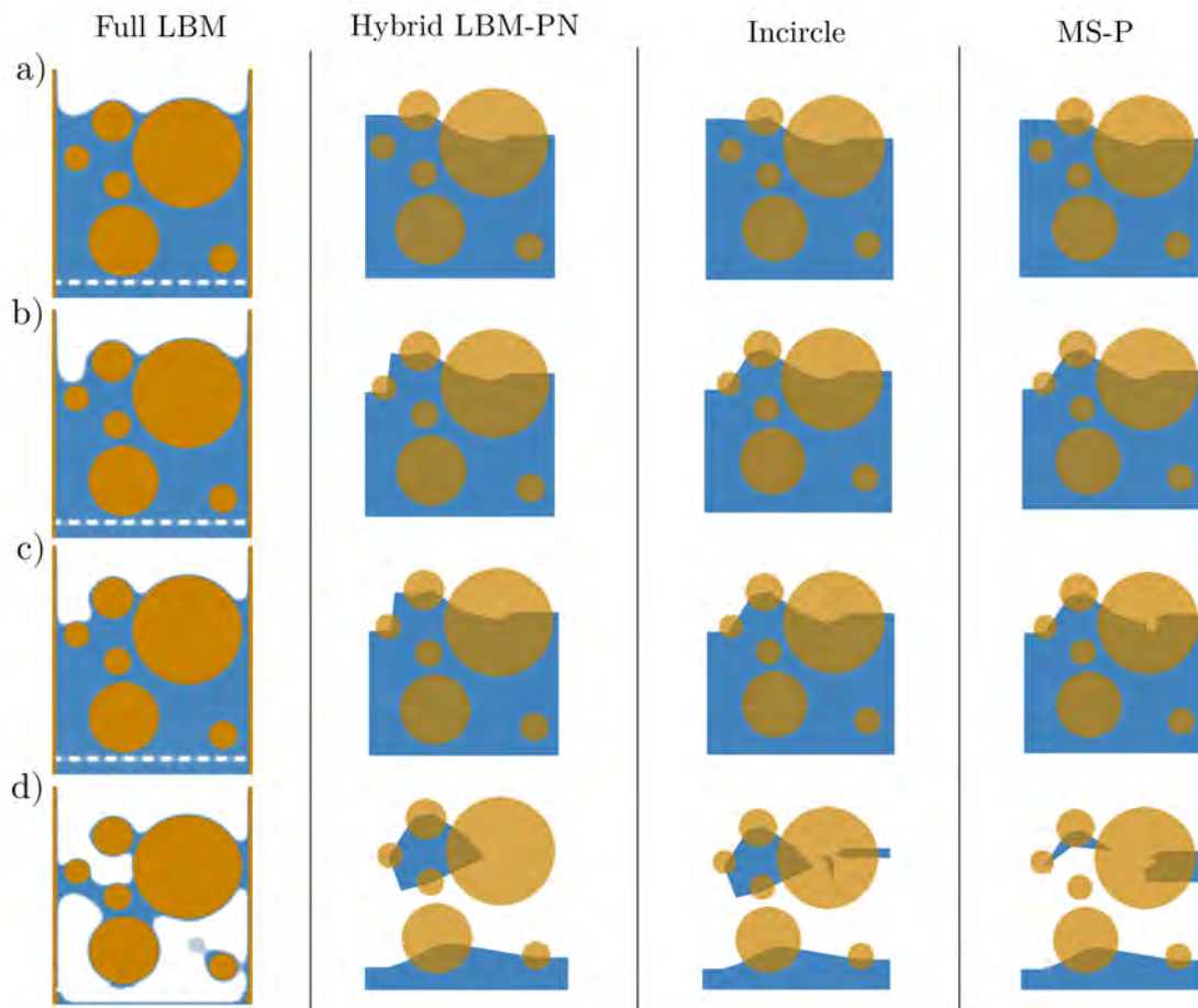
Figure 6.17: Comparison of the invasion path for plane B (see figure 6.15). a) p_c^* = 2.4 , b) p_c^* = 3.3 , c) p_c^* = 4.2 and d) p_c^* = 5.3 .
