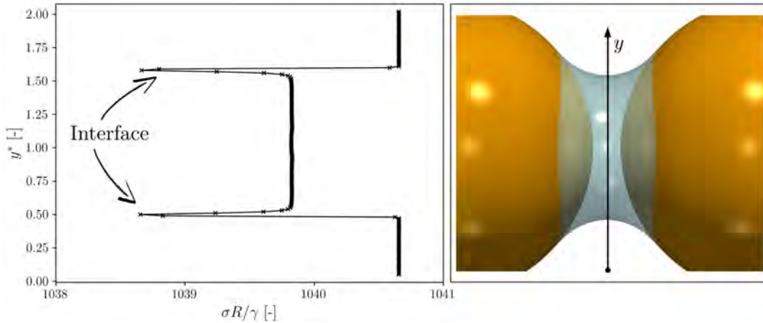
Figure 3.2: Horizontal stress along the vertical axis.
