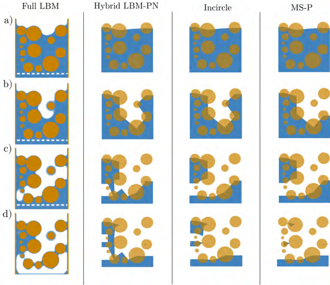
Figure 6.18: Comparison of the invasion path for plane C (see figure 6.15). a) p_c^* = 2.4 , b) p_c^* = 3.3 , c) p_c^* = 4.2 and d) p_c^* = 5.3 .
