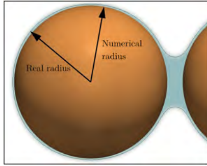
Figure 2.11: Principle of the wall retraction method. In the LBM mesh the solid boundary is retracted by 2lu with respect to its real position, such that the fluid-fluid contour \rho_w / \rho_o = 0.7 is nearly coincident with the real boundary.
